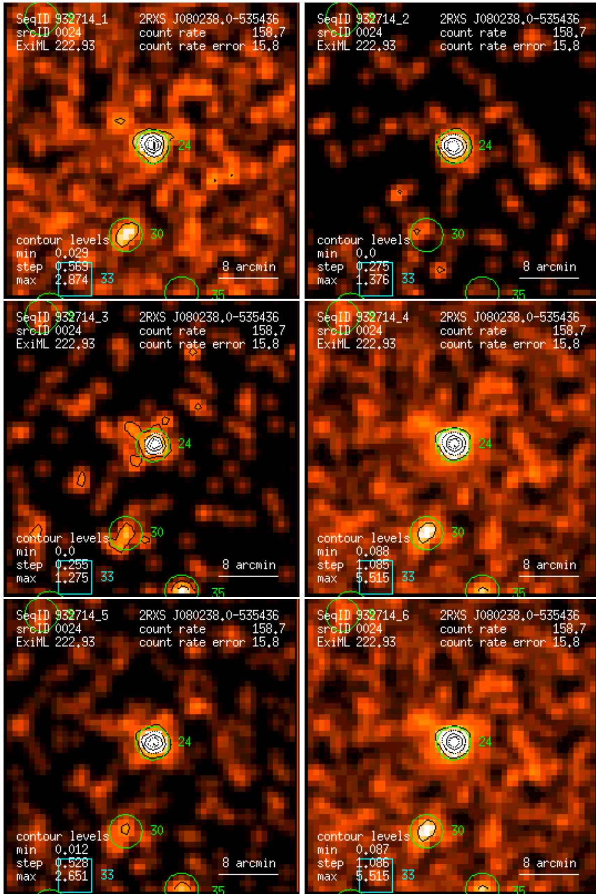
Figure 24: RASS 932714: detection 0024: band rate images, Gaussian filter: (1) PSPC channels 11 – 41, (2) 52 – 90, (3) 91 – 201, (4) 11 – 235, (5) 52 – 201, (6) 11 – 201. Broad band rates in counts/ks. Band rate contour levels in counts/ks/arcmin 2 .
