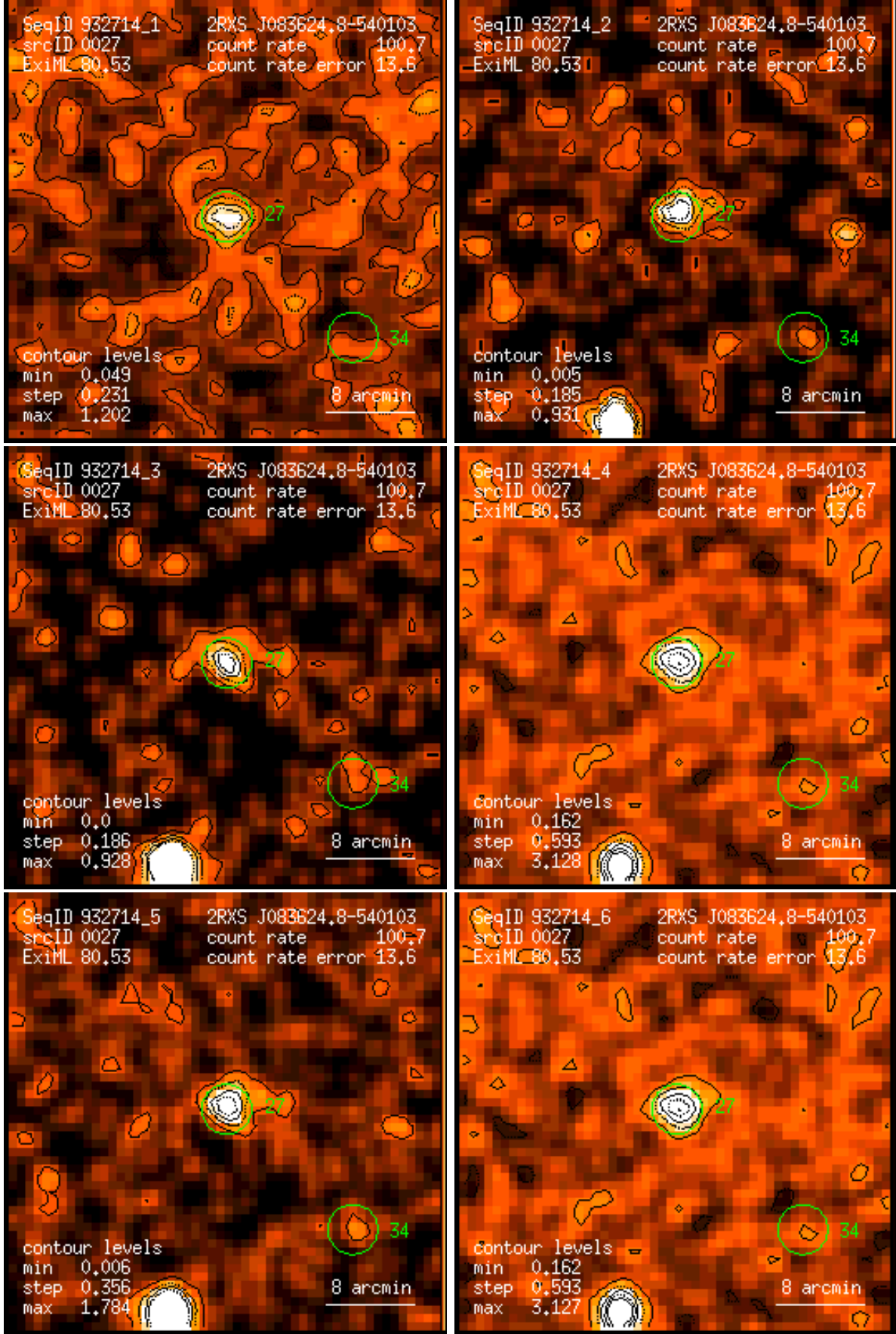
Figure 27: RASS 932714: detection 0027: band rate images, Gaussian filter: (1) PSPC channels 11 – 41, (2) 52 – 90, (3) 91 – 201, (4) 11 – 235, (5) 52 – 201, (6) 11 – 201. Broad band rates in counts/ks. Band rate contour levels in counts/ks/arcmin 2 .
