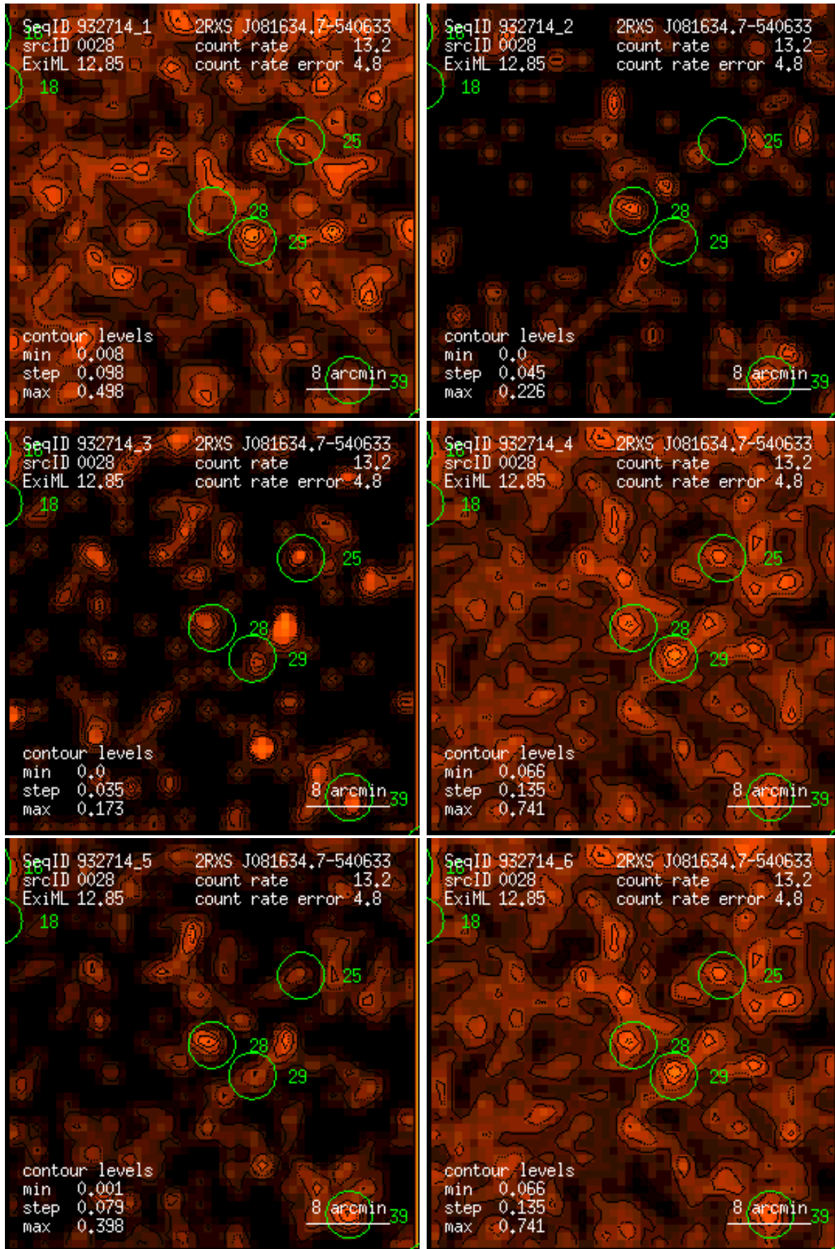
Figure 28: RASS 932714: detection 0028: band rate images, Gaussian filter: (1) PSPC channels 11 – 41, (2) 52 – 90, (3) 91 – 201, (4) 11 – 235, (5) 52 – 201, (6) 11 – 201. Broad band rates in counts/ks. Band rate contour levels in counts/ks/arcmin 2 .
