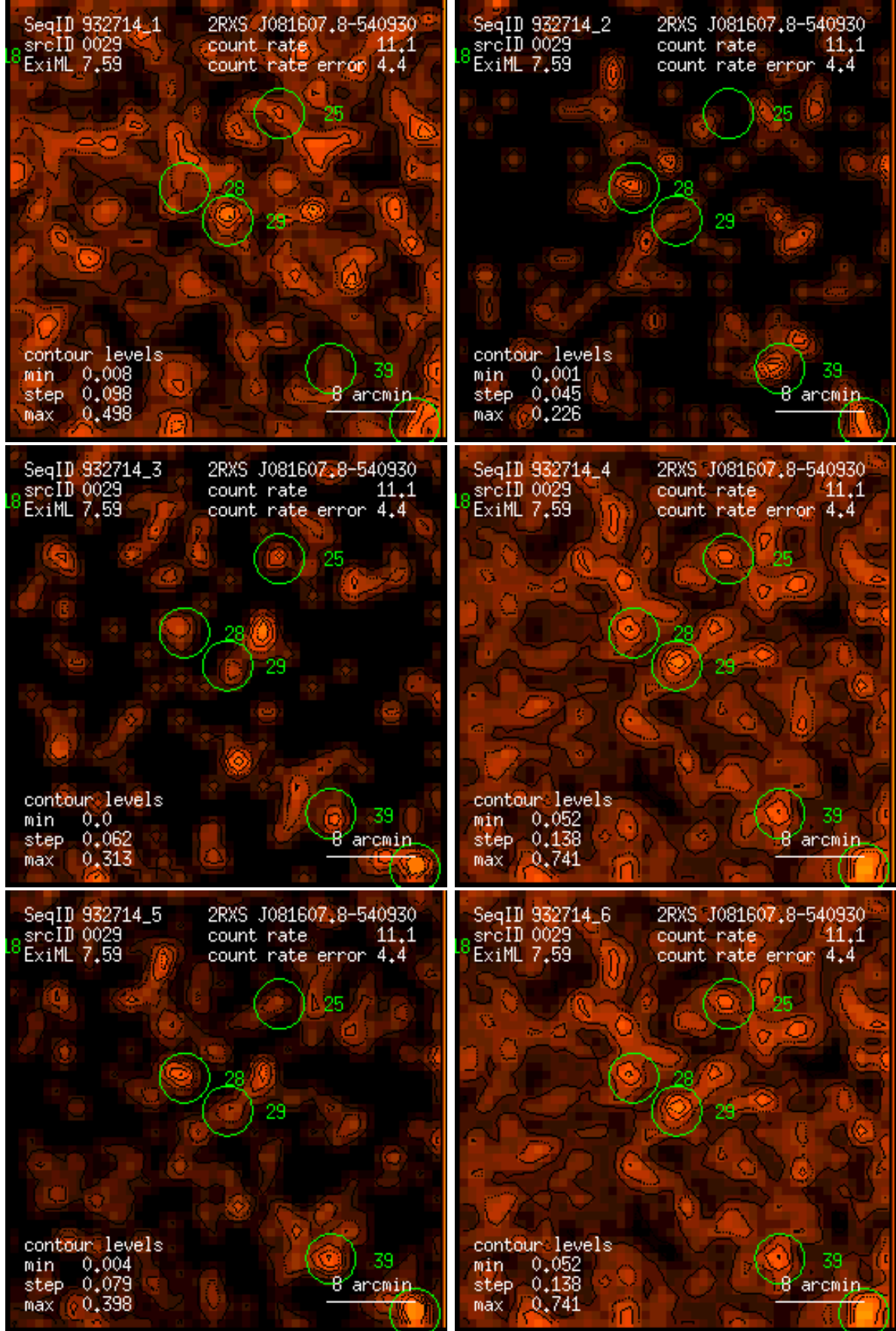
Figure 29: RASS 932714: detection 0029: band rate images, Gaussian filter: (1) PSPC channels 11 – 41, (2) 52 – 90, (3) 91 – 201, (4) 11 – 235, (5) 52 – 201, (6) 11 – 201. Broad band rates in counts/ks. Band rate contour levels in counts/ks/arcmin 2 .
