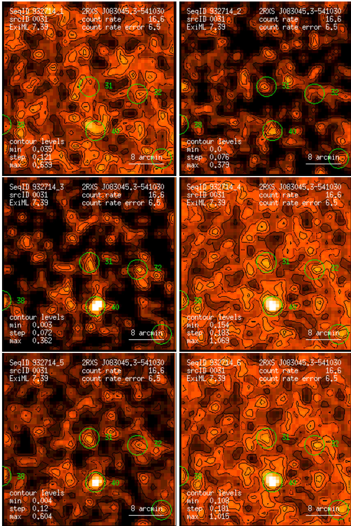
Figure 31: RASS 932714: detection 0031: band rate images, Gaussian filter: (1) PSPC channels 11 – 41, (2) 52 – 90, (3) 91 – 201, (4) 11 – 235, (5) 52 – 201, (6) 11 – 201. Broad band rates in counts/ks. Band rate contour levels in counts/ks/arcmin 2 .
