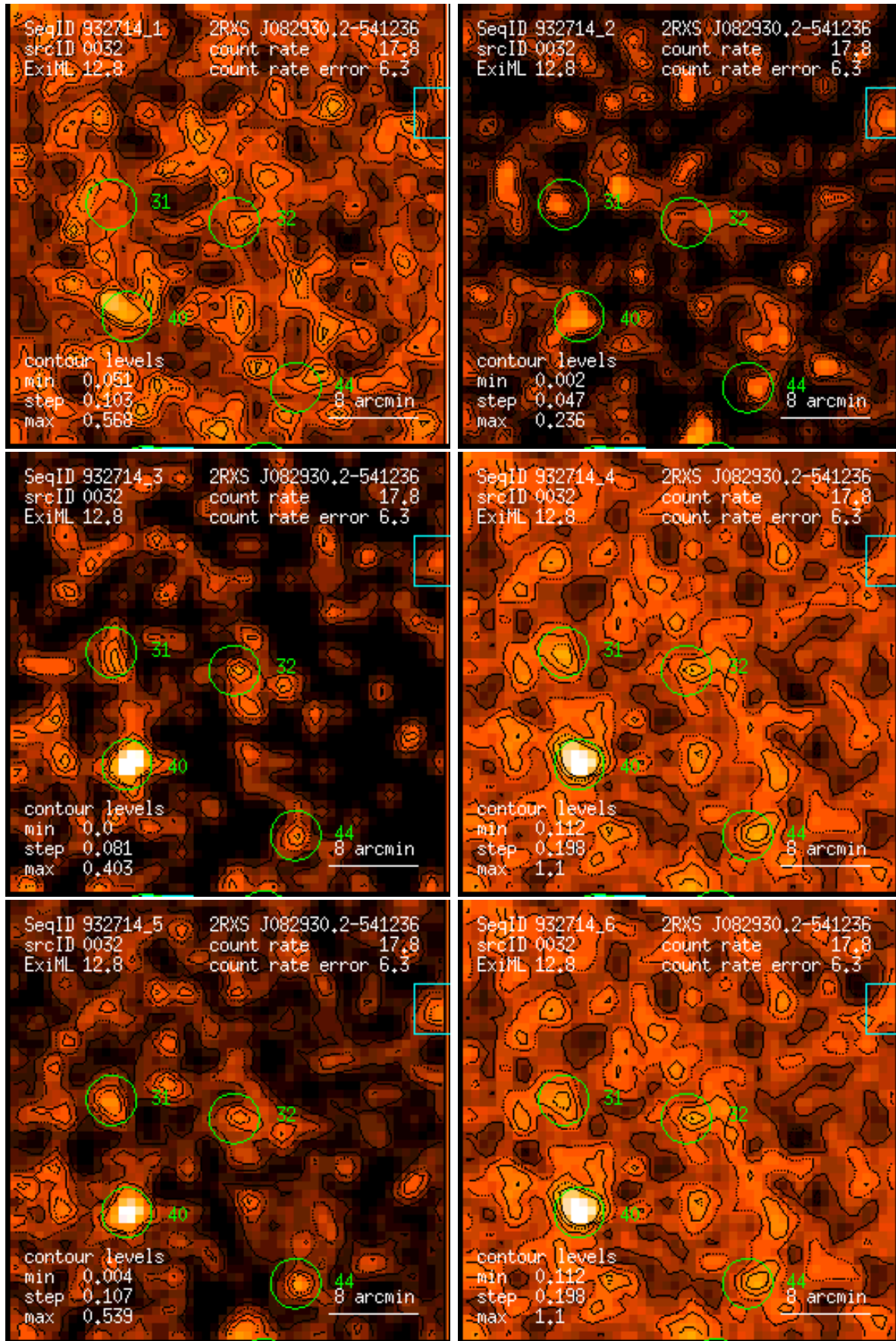
Figure 32: RASS 932714: detection 0032: band rate images, Gaussian filter: (1) PSPC channels 11 – 41, (2) 52 – 90, (3) 91 – 201, (4) 11 – 235, (5) 52 – 201, (6) 11 – 201. Broad band rates in counts/ks. Band rate contour levels in counts/ks/arcmin 2 .
