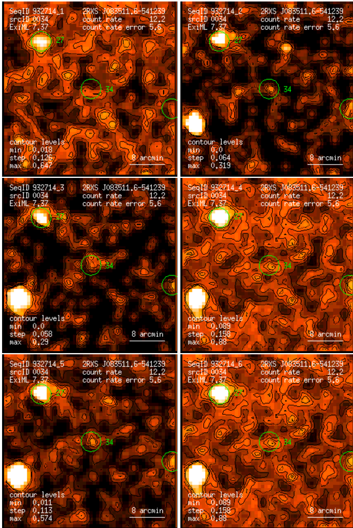
Figure 34: RASS 932714: detection 0034: band rate images, Gaussian filter: (1) PSPC channels 11 – 41, (2) 52 – 90, (3) 91 – 201, (4) 11 – 235, (5) 52 – 201, (6) 11 – 201. Broad band rates in counts/ks. Band rate contour levels in counts/ks/arcmin 2 .
