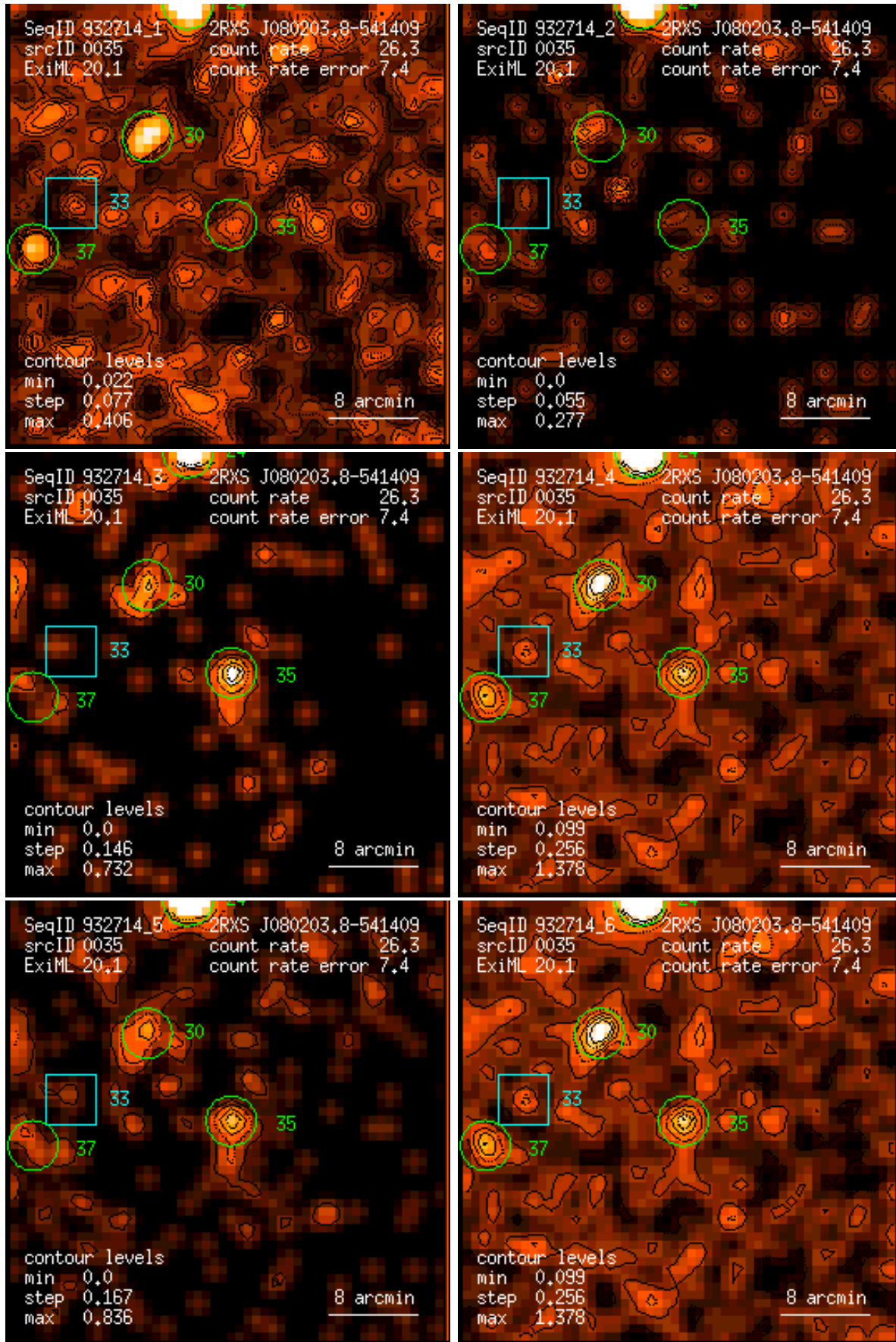
Figure 35: RASS 932714: detection 0035: band rate images, Gaussian filter: (1) PSPC channels 11 – 41, (2) 52 – 90, (3) 91 – 201, (4) 11 – 235, (5) 52 – 201, (6) 11 – 201. Broad band rates in counts/ks. Band rate contour levels in counts/ks/arcmin 2 .
