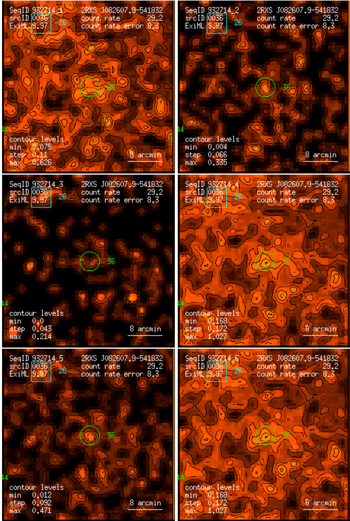
Figure 36: RASS 932714: detection 0036: band rate images, Gaussian filter: (1) PSPC channels 11 – 41, (2) 52 – 90, (3) 91 – 201, (4) 11 – 235, (5) 52 – 201, (6) 11 – 201. Broad band rates in counts/ks. Band rate contour levels in counts/ks/arcmin 2 .
