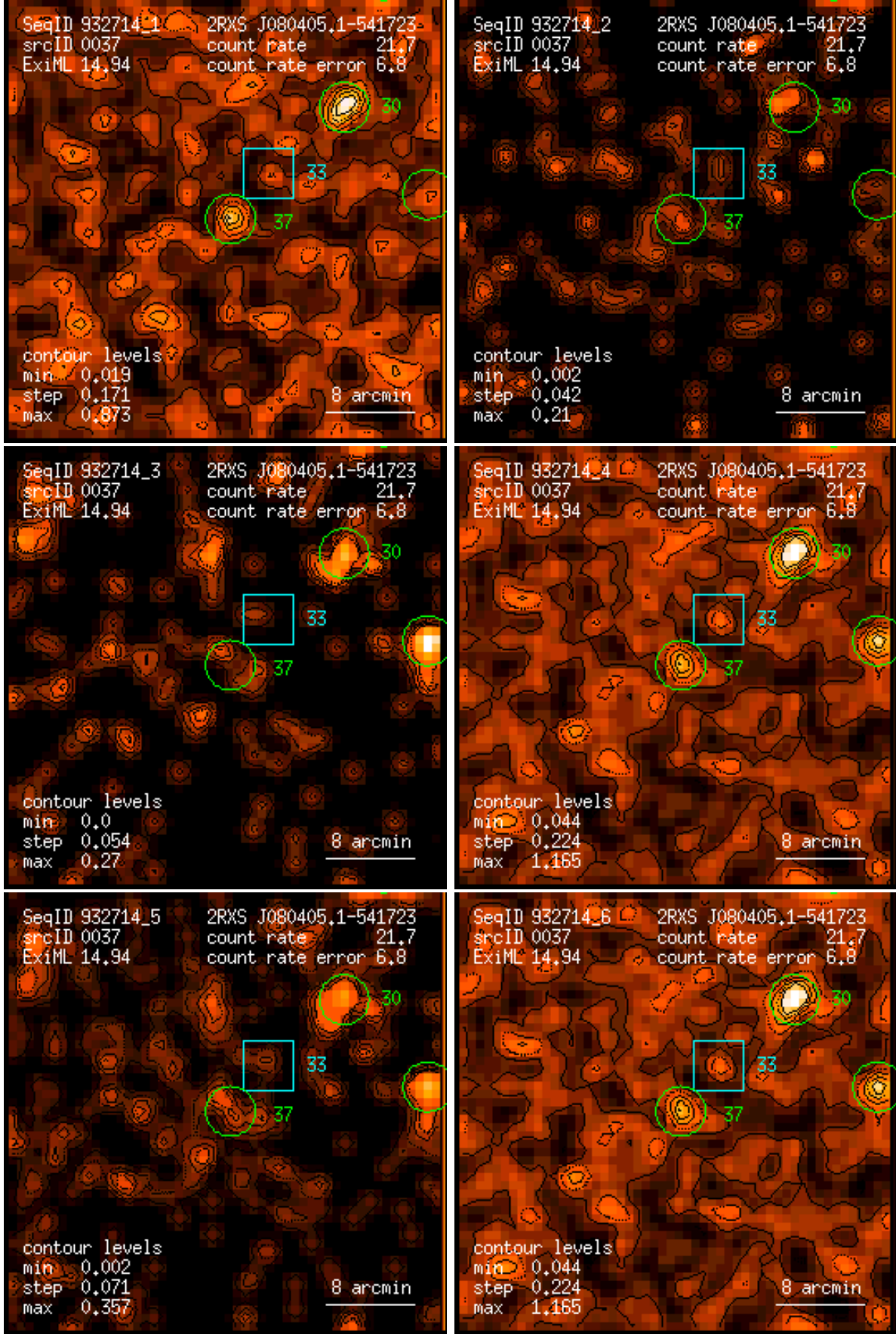
Figure 37: RASS 932714: detection 0037: band rate images, Gaussian filter: (1) PSPC channels 11 – 41, (2) 52 – 90, (3) 91 – 201, (4) 11 – 235, (5) 52 – 201, (6) 11 – 201. Broad band rates in counts/ks. Band rate contour levels in counts/ks/arcmin 2 .
