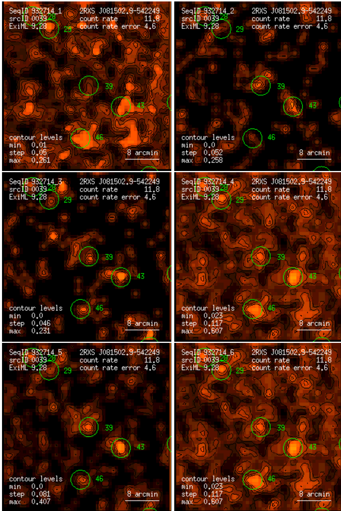
Figure 39: RASS 932714: detection 0039: band rate images, Gaussian filter: (1) PSPC channels 11 – 41, (2) 52 – 90, (3) 91 – 201, (4) 11 – 235, (5) 52 – 201, (6) 11 – 201. Broad band rates in counts/ks. Band rate contour levels in counts/ks/arcmin 2 .
