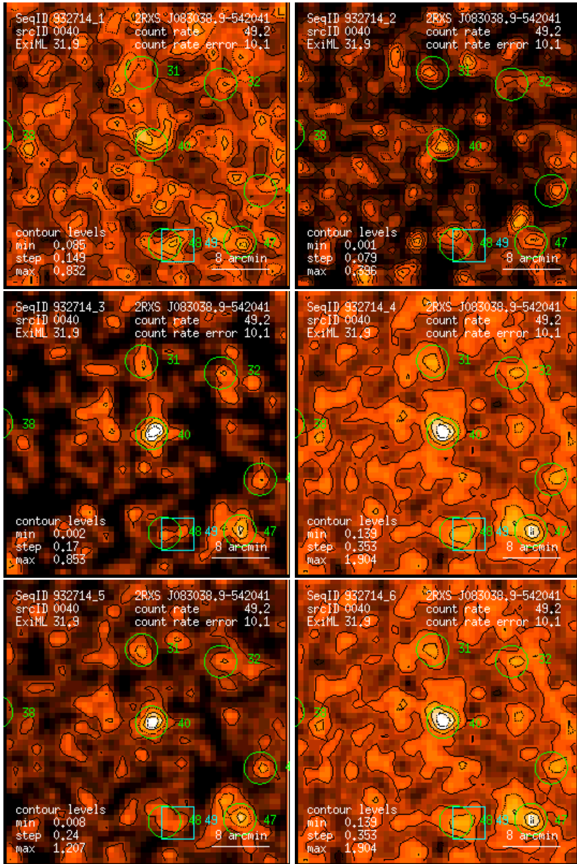
Figure 40: RASS 932714: detection 0040: band rate images, Gaussian filter: (1) PSPC channels 11 – 41, (2) 52 – 90, (3) 91 – 201, (4) 11 – 235, (5) 52 – 201, (6) 11 – 201. Broad band rates in counts/ks. Band rate contour levels in counts/ks/arcmin 2 .
