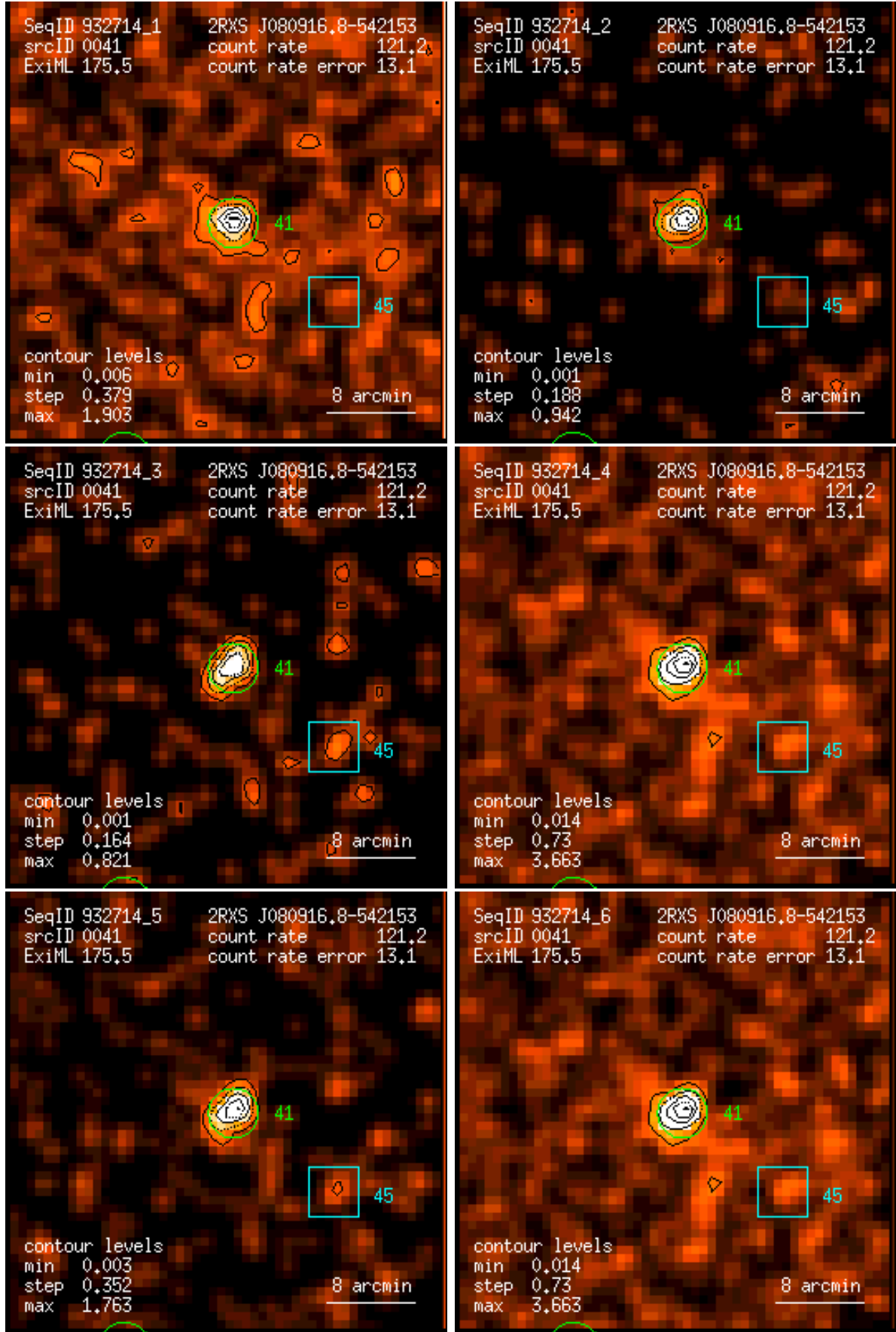
Figure 41: RASS 932714: detection 0041: band rate images, Gaussian filter: (1) PSPC channels 11 – 41, (2) 52 – 90, (3) 91 – 201, (4) 11 – 235, (5) 52 – 201, (6) 11 – 201. Broad band rates in counts/ks. Band rate contour levels in counts/ks/arcmin 2 .
