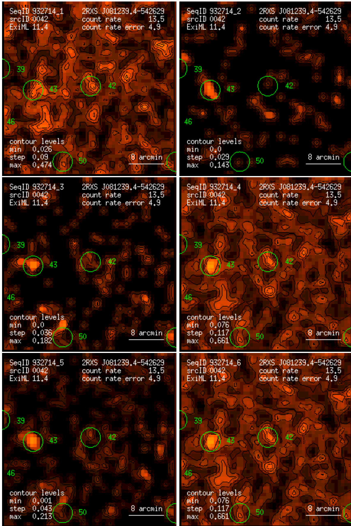
Figure 42: RASS 932714: detection 0042: band rate images, Gaussian filter: (1) PSPC channels 11 – 41, (2) 52 – 90, (3) 91 – 201, (4) 11 – 235, (5) 52 – 201, (6) 11 – 201. Broad band rates in counts/ks. Band rate contour levels in counts/ks/arcmin 2 .
