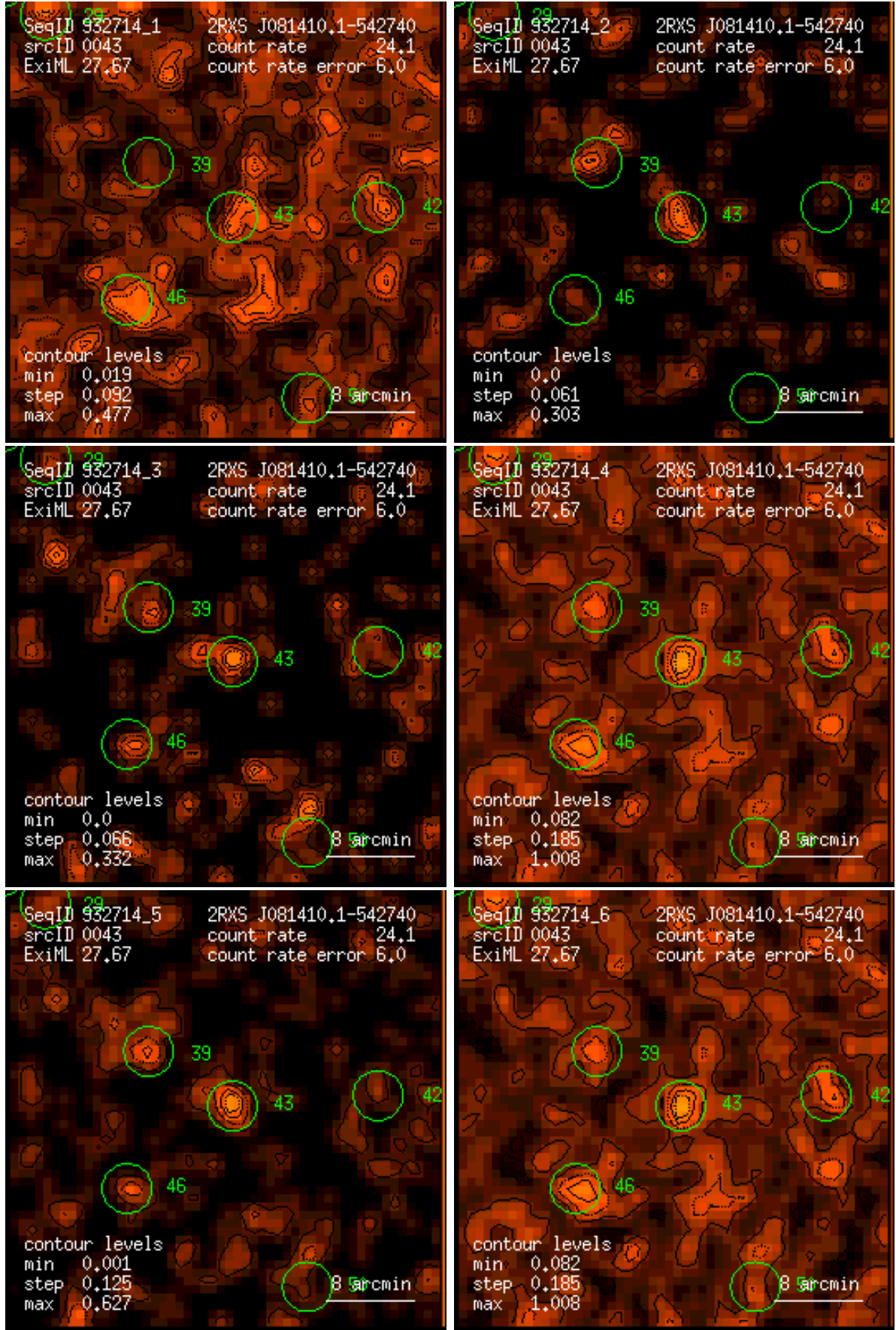
Figure 43: RASS 932714: detection 0043: band rate images, Gaussian filter: (1) PSPC channels 11 – 41, (2) 52 – 90, (3) 91 – 201, (4) 11 – 235, (5) 52 – 201, (6) 11 – 201. Broad band rates in counts/ks. Band rate contour levels in counts/ks/arcmin 2 .
