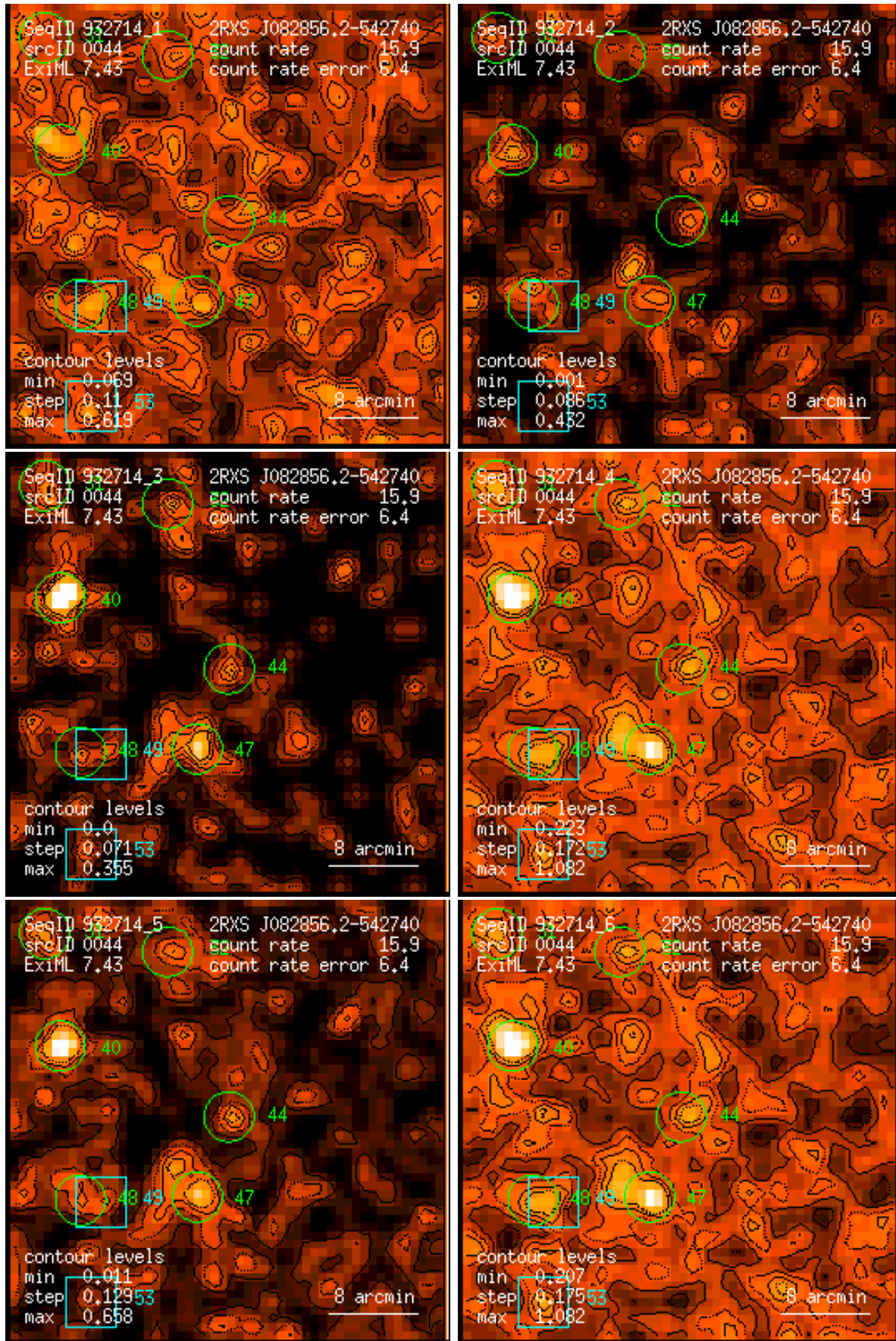
Figure 44: RASS 932714: detection 0044: band rate images, Gaussian filter: (1) PSPC channels 11 – 41, (2) 52 – 90, (3) 91 – 201, (4) 11 – 235, (5) 52 – 201, (6) 11 – 201. Broad band rates in counts/ks. Band rate contour levels in counts/ks/arcmin 2 .
