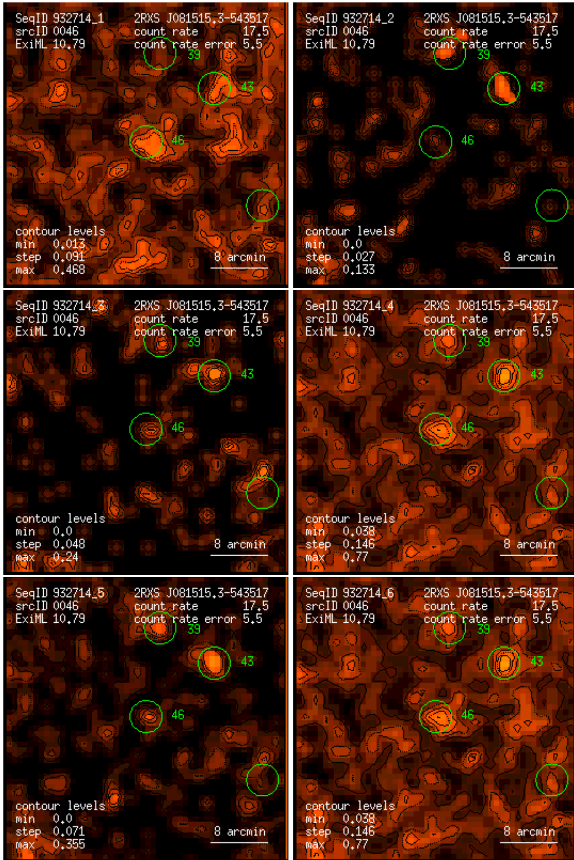
Figure 46: RASS 932714: detection 0046: band rate images, Gaussian filter: (1) PSPC channels 11 – 41, (2) 52 – 90, (3) 91 – 201, (4) 11 – 235, (5) 52 – 201, (6) 11 – 201. Broad band rates in counts/ks. Band rate contour levels in counts/ks/arcmin 2 .
