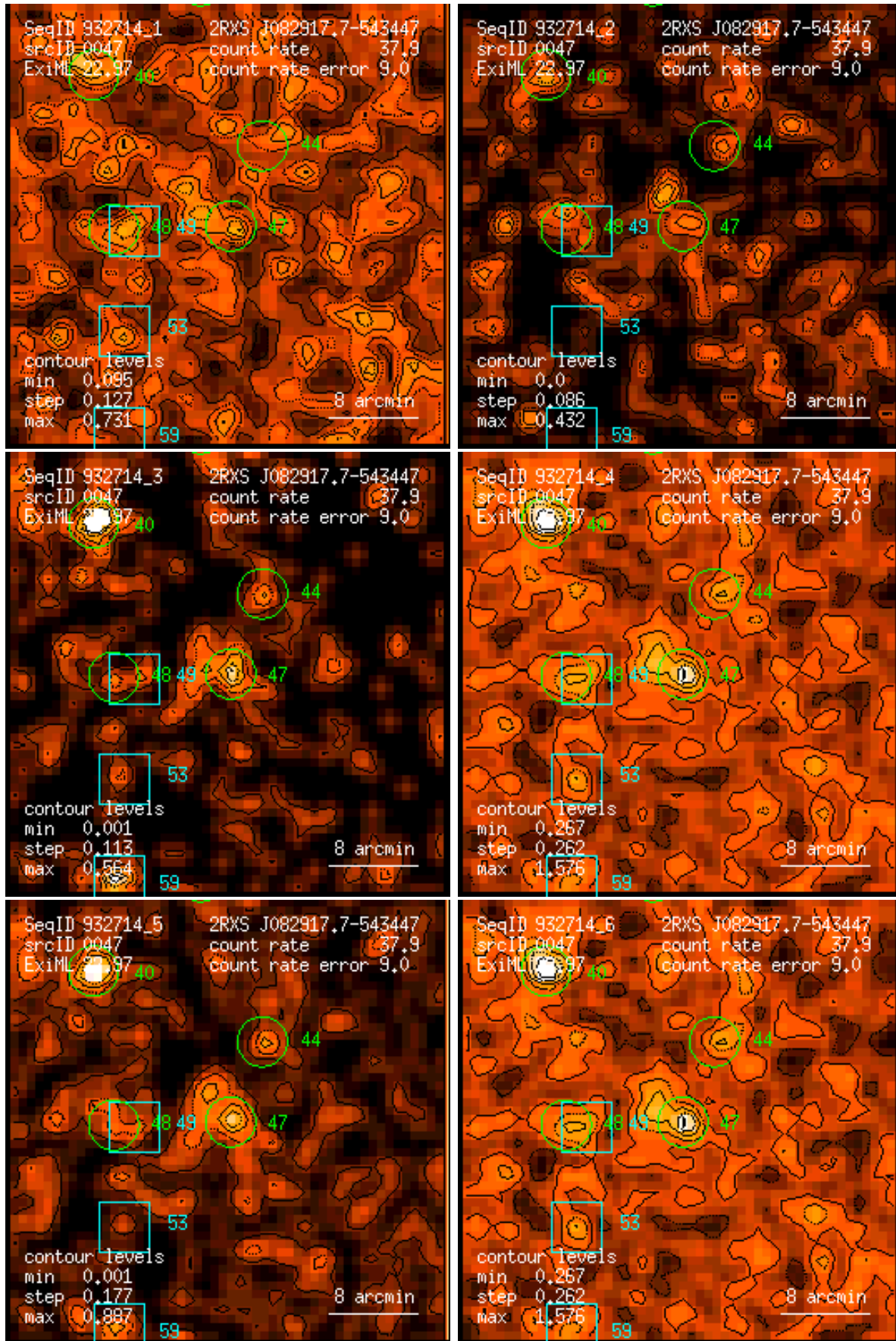
Figure 47: RASS 932714: detection 0047: band rate images, Gaussian filter: (1) PSPC channels 11 – 41, (2) 52 – 90, (3) 91 – 201, (4) 11 – 235, (5) 52 – 201, (6) 11 – 201. Broad band rates in counts/ks. Band rate contour levels in counts/ks/arcmin 2 .
