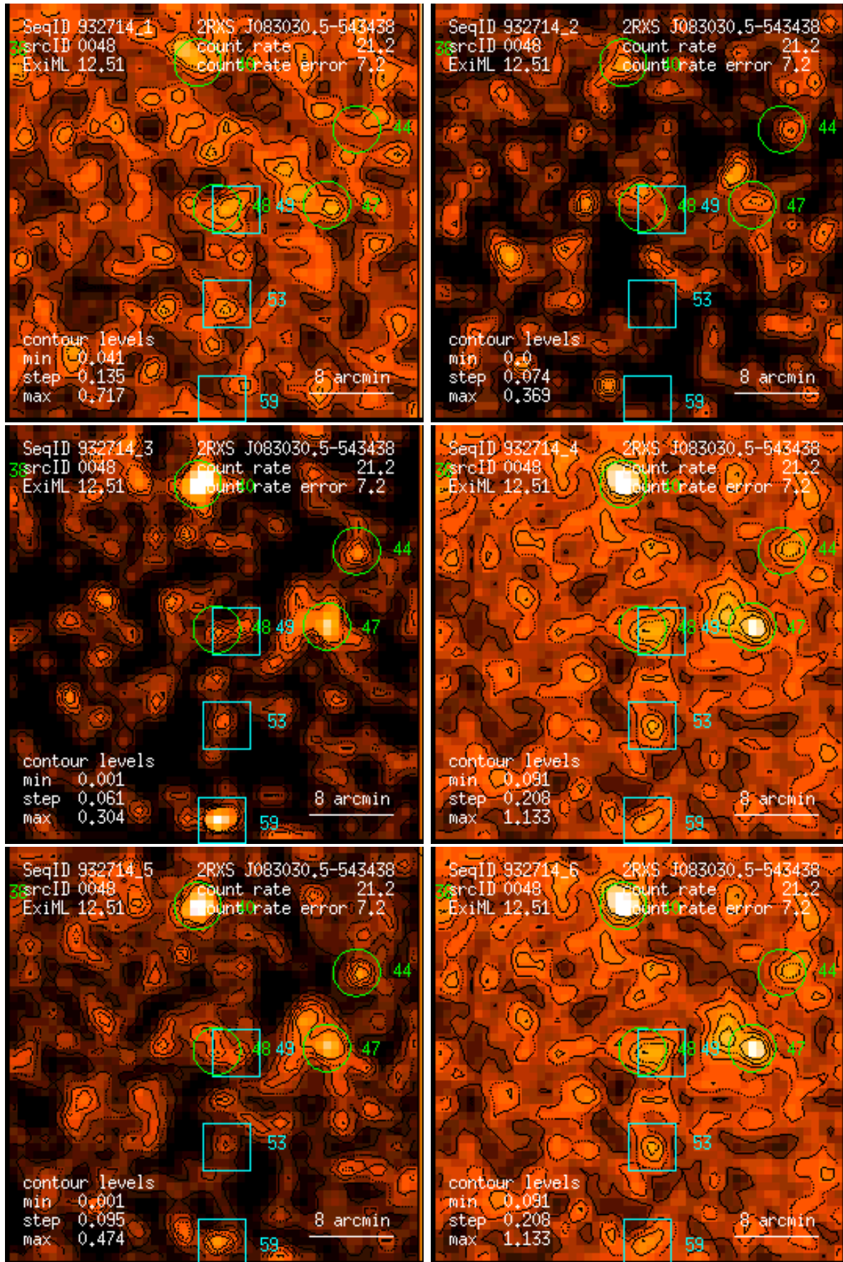
Figure 48: RASS 932714: detection 0048: band rate images, Gaussian filter: (1) PSPC channels 11 – 41, (2) 52 – 90, (3) 91 – 201, (4) 11 – 235, (5) 52 – 201, (6) 11 – 201. Broad band rates in counts/ks. Band rate contour levels in counts/ks/arcmin 2 .
