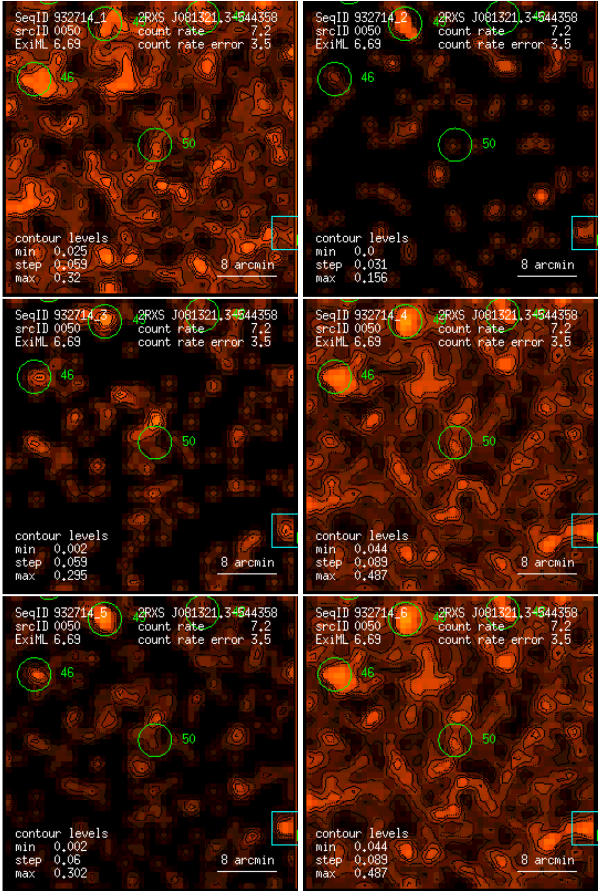
Figure 50: RASS 932714: detection 0050: band rate images, Gaussian filter: (1) PSPC channels 11 – 41, (2) 52 – 90, (3) 91 – 201, (4) 11 – 235, (5) 52 – 201, (6) 11 – 201. Broad band rates in counts/ks. Band rate contour levels in counts/ks/arcmin 2 .
