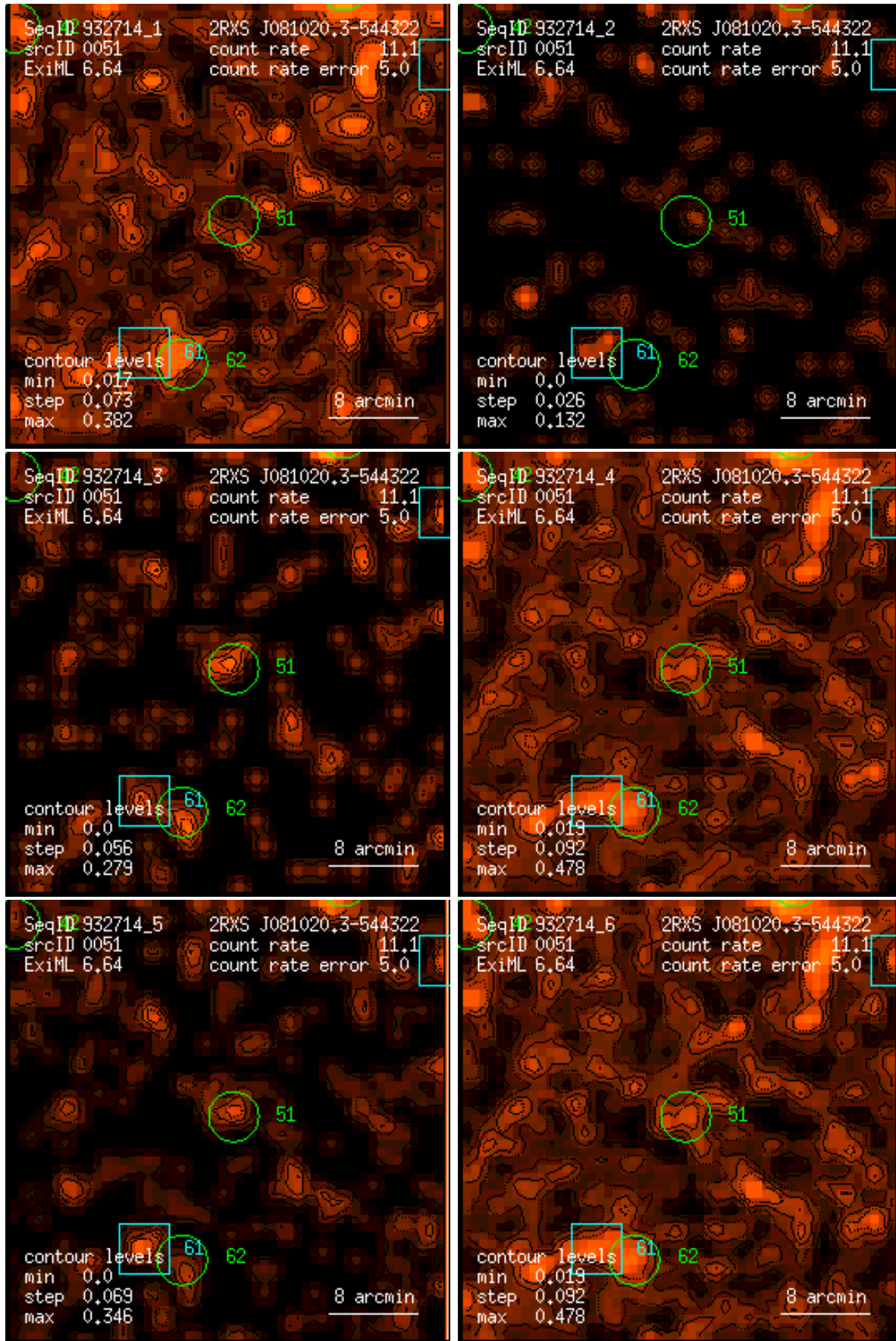
Figure 51: RASS 932714: detection 0051: band rate images, Gaussian filter: (1) PSPC channels 11 – 41, (2) 52 – 90, (3) 91 – 201, (4) 11 – 235, (5) 52 – 201, (6) 11 – 201. Broad band rates in counts/ks. Band rate contour levels in counts/ks/arcmin 2 .
