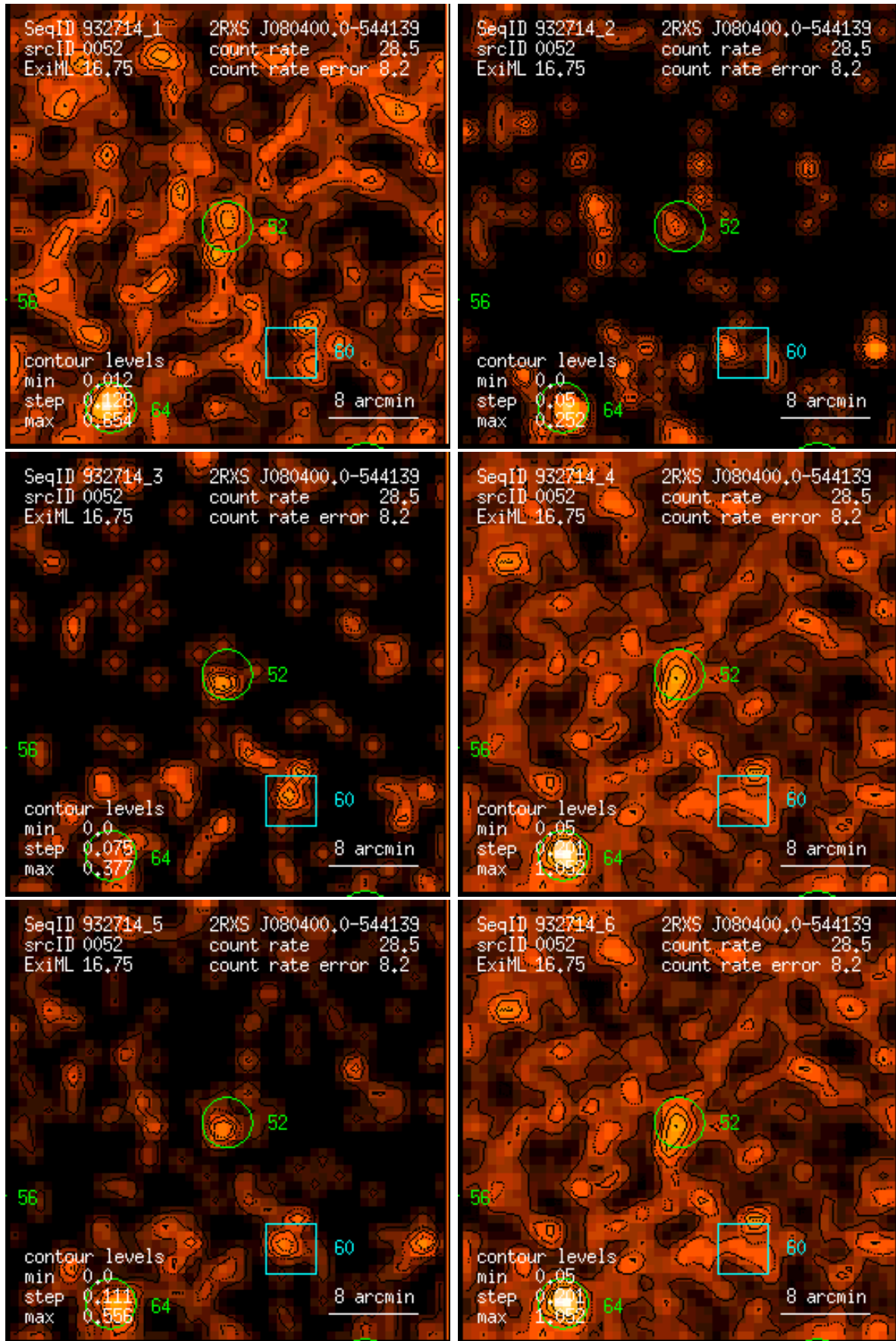
Figure 52: RASS 932714: detection 0052: band rate images, Gaussian filter: (1) PSPC channels 11 – 41, (2) 52 – 90, (3) 91 – 201, (4) 11 – 235, (5) 52 – 201, (6) 11 – 201. Broad band rates in counts/ks. Band rate contour levels in counts/ks/arcmin 2 .
