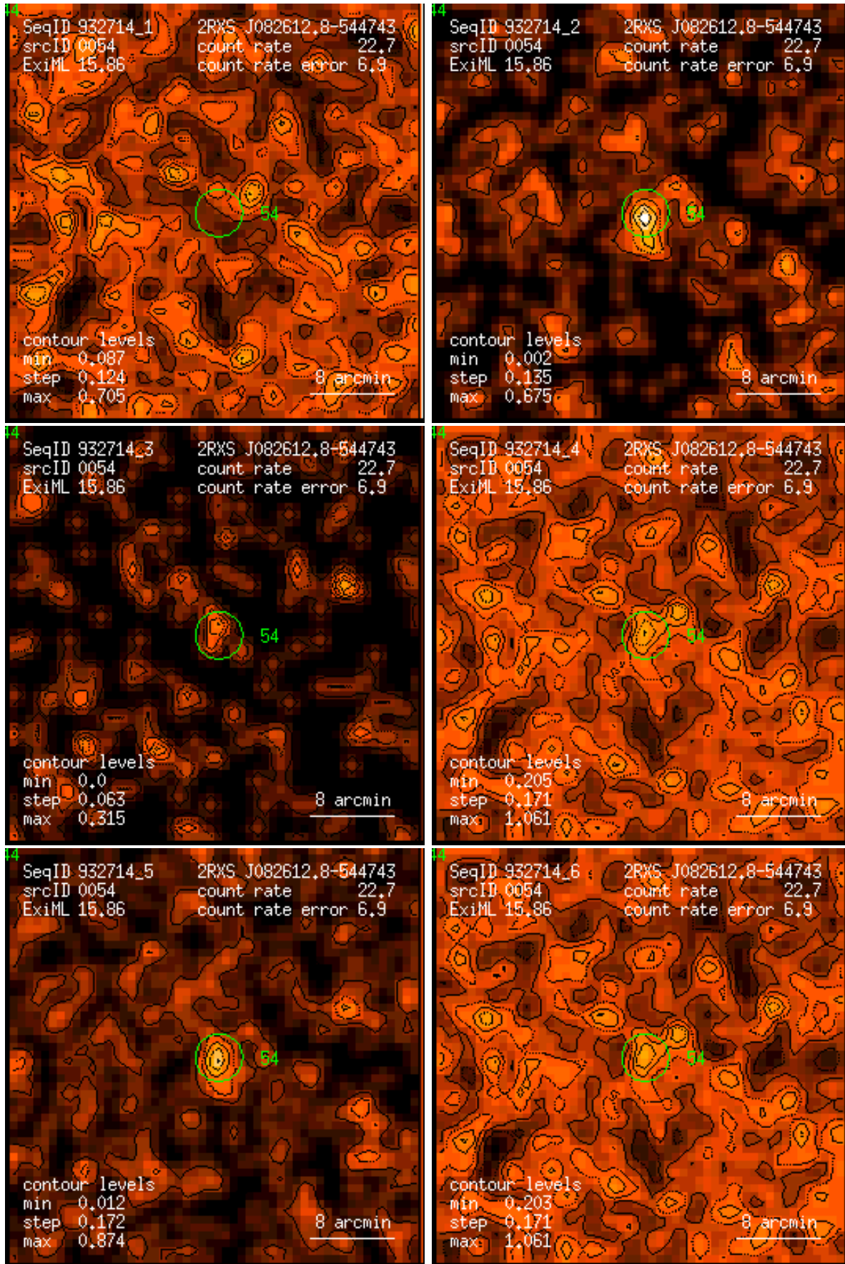
Figure 54: RASS 932714: detection 0054: band rate images, Gaussian filter: (1) PSPC channels 11 – 41, (2) 52 – 90, (3) 91 – 201, (4) 11 – 235, (5) 52 – 201, (6) 11 – 201. Broad band rates in counts/ks. Band rate contour levels in counts/ks/arcmin 2 .
