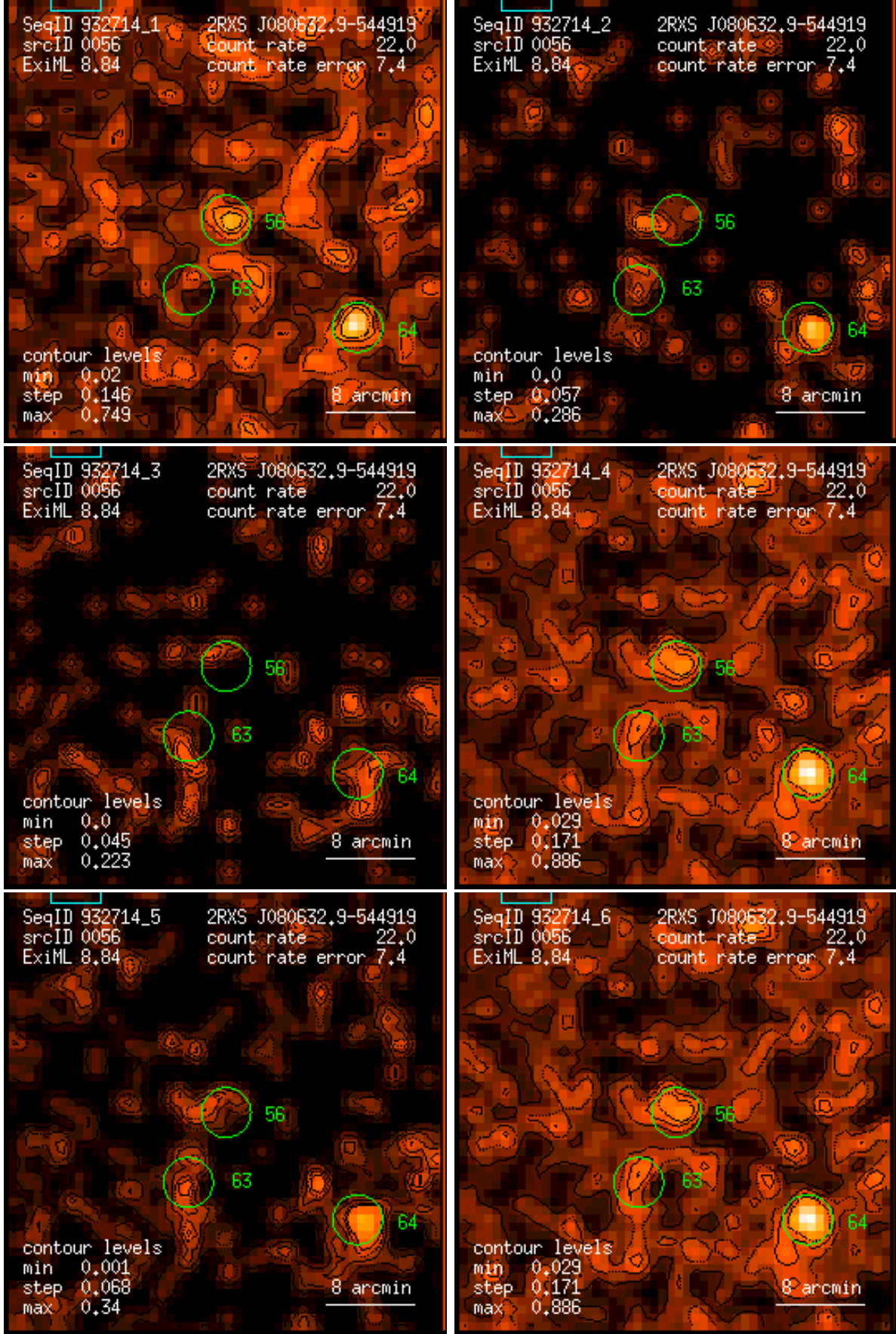
Figure 56: RASS 932714: detection 0056: band rate images, Gaussian filter: (1) PSPC channels 11 – 41, (2) 52 – 90, (3) 91 – 201, (4) 11 – 235, (5) 52 – 201, (6) 11 – 201. Broad band rates in counts/ks. Band rate contour levels in counts/ks/arcmin 2 .
