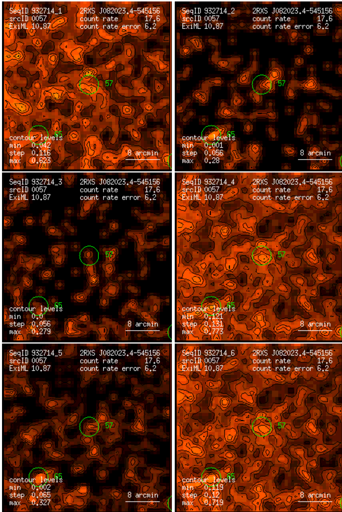
Figure 57: RASS 932714: detection 0057: band rate images, Gaussian filter: (1) PSPC channels 11 – 41, (2) 52 – 90, (3) 91 – 201, (4) 11 – 235, (5) 52 – 201, (6) 11 – 201. Broad band rates in counts/ks. Band rate contour levels in counts/ks/arcmin 2 .
