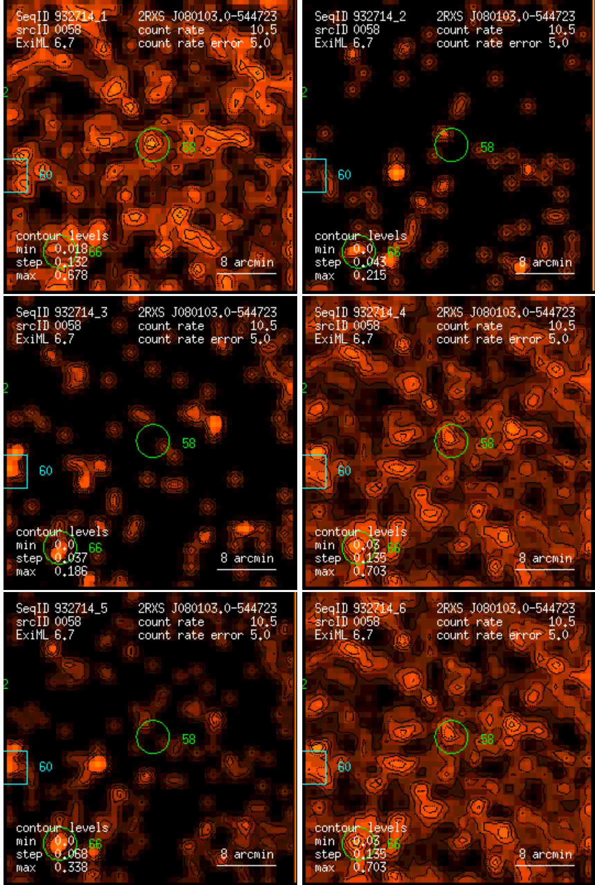
Figure 58: RASS 932714: detection 0058: band rate images, Gaussian filter: (1) PSPC channels 11 – 41, (2) 52 – 90, (3) 91 – 201, (4) 11 – 235, (5) 52 – 201, (6) 11 – 201. Broad band rates in counts/ks. Band rate contour levels in counts/ks/arcmin 2 .
