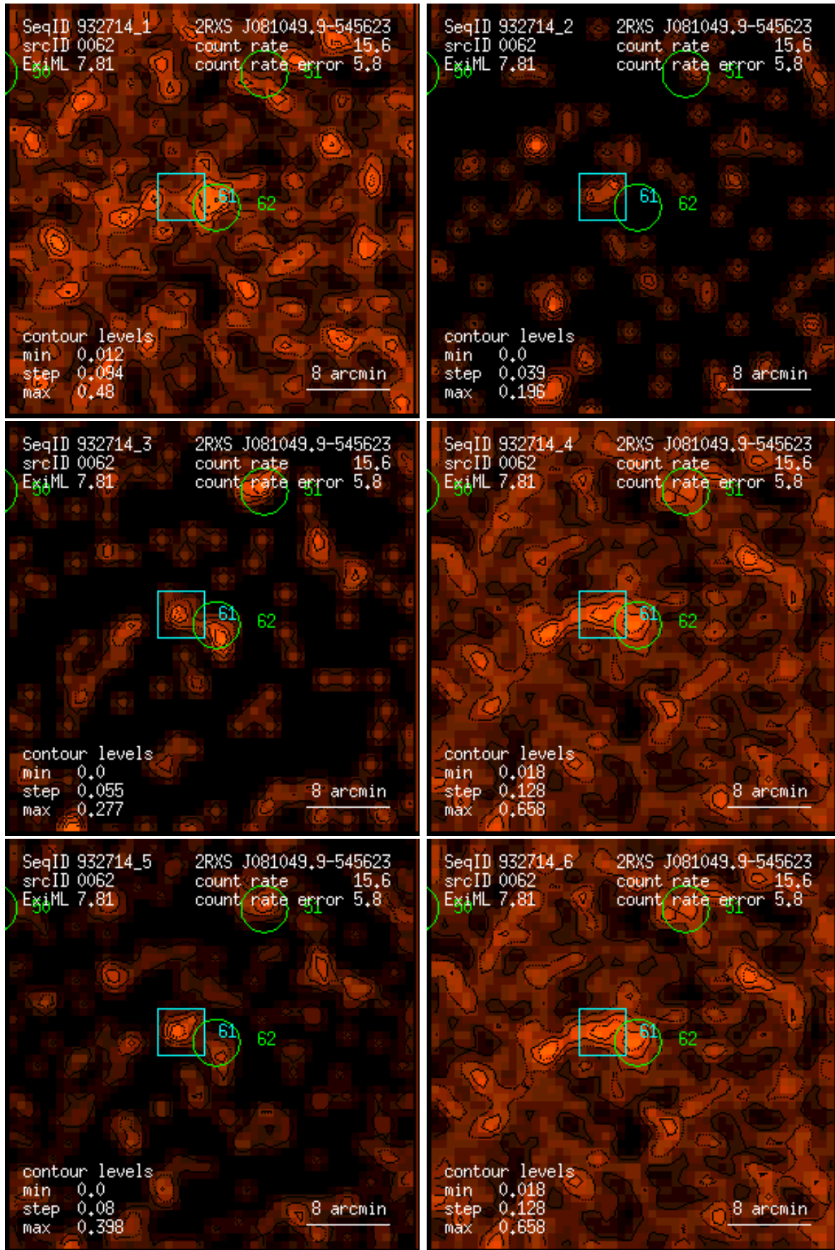
Figure 62: RASS 932714: detection 0062: band rate images, Gaussian filter: (1) PSPC channels 11 – 41, (2) 52 – 90, (3) 91 – 201, (4) 11 – 235, (5) 52 – 201, (6) 11 – 201. Broad band rates in counts/ks. Band rate contour levels in counts/ks/arcmin 2 .
