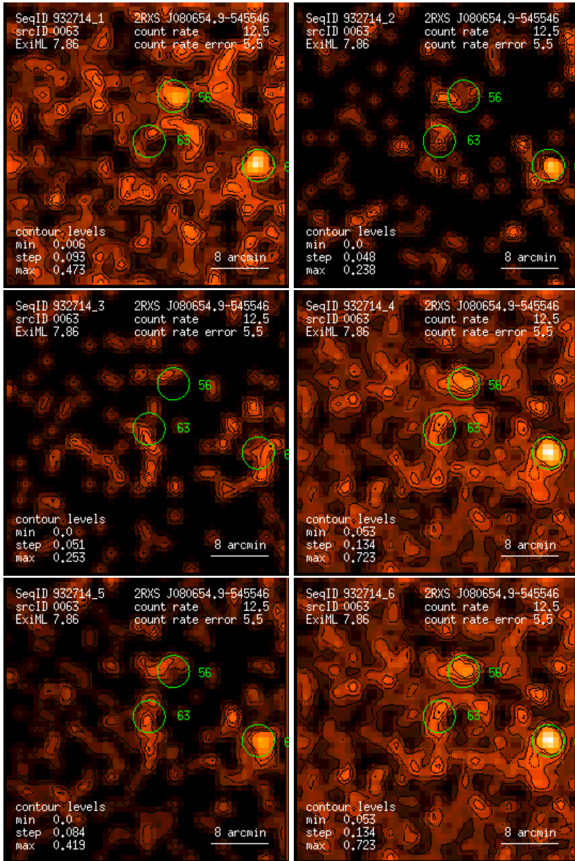
Figure 63: RASS 932714: detection 0063: band rate images, Gaussian filter: (1) PSPC channels 11 – 41, (2) 52 – 90, (3) 91 – 201, (4) 11 – 235, (5) 52 – 201, (6) 11 – 201. Broad band rates in counts/ks. Band rate contour levels in counts/ks/arcmin 2 .
