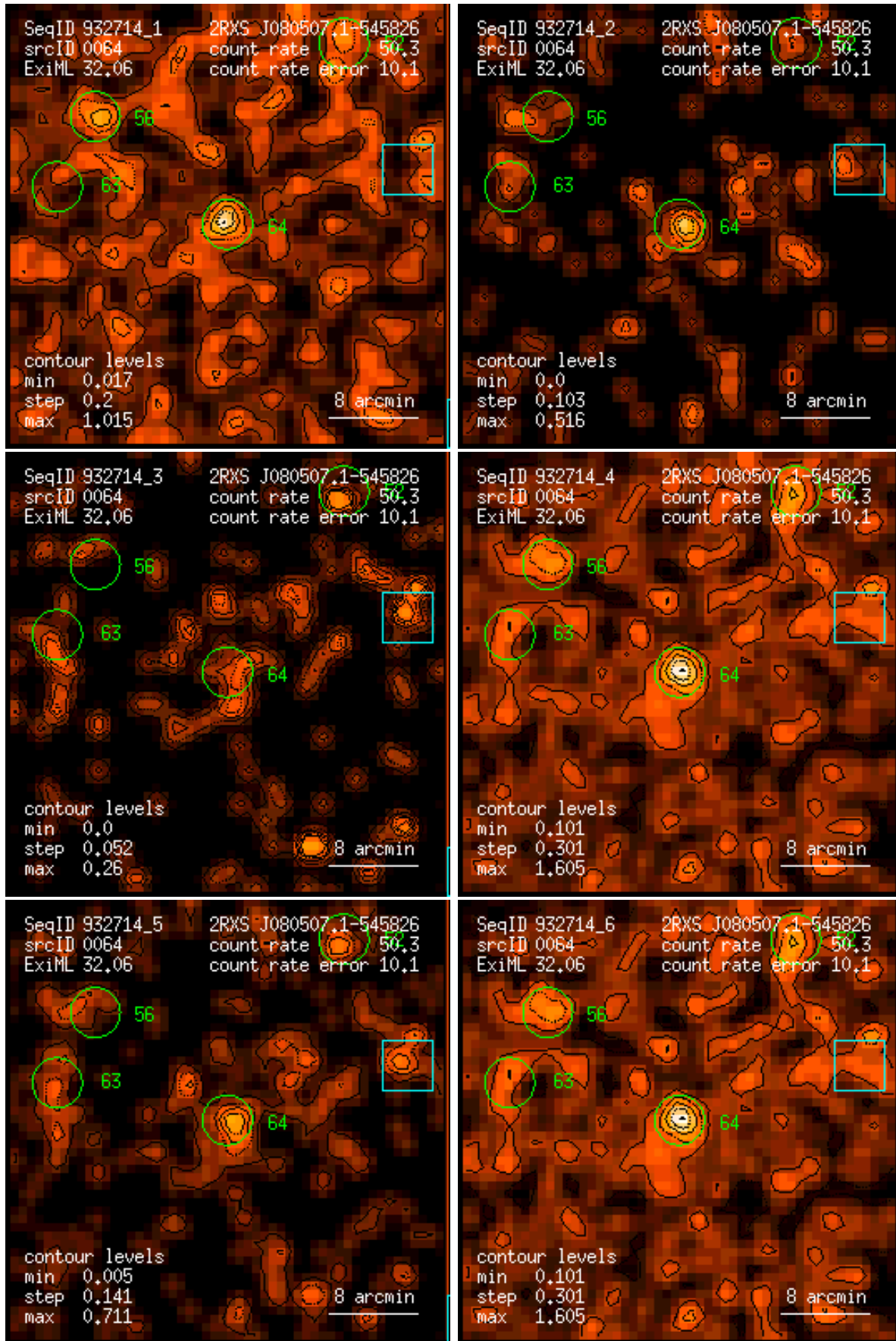
Figure 64: RASS 932714: detection 0064: band rate images, Gaussian filter: (1) PSPC channels 11 – 41, (2) 52 – 90, (3) 91 – 201, (4) 11 – 235, (5) 52 – 201, (6) 11 – 201. Broad band rates in counts/ks. Band rate contour levels in counts/ks/arcmin 2 .
