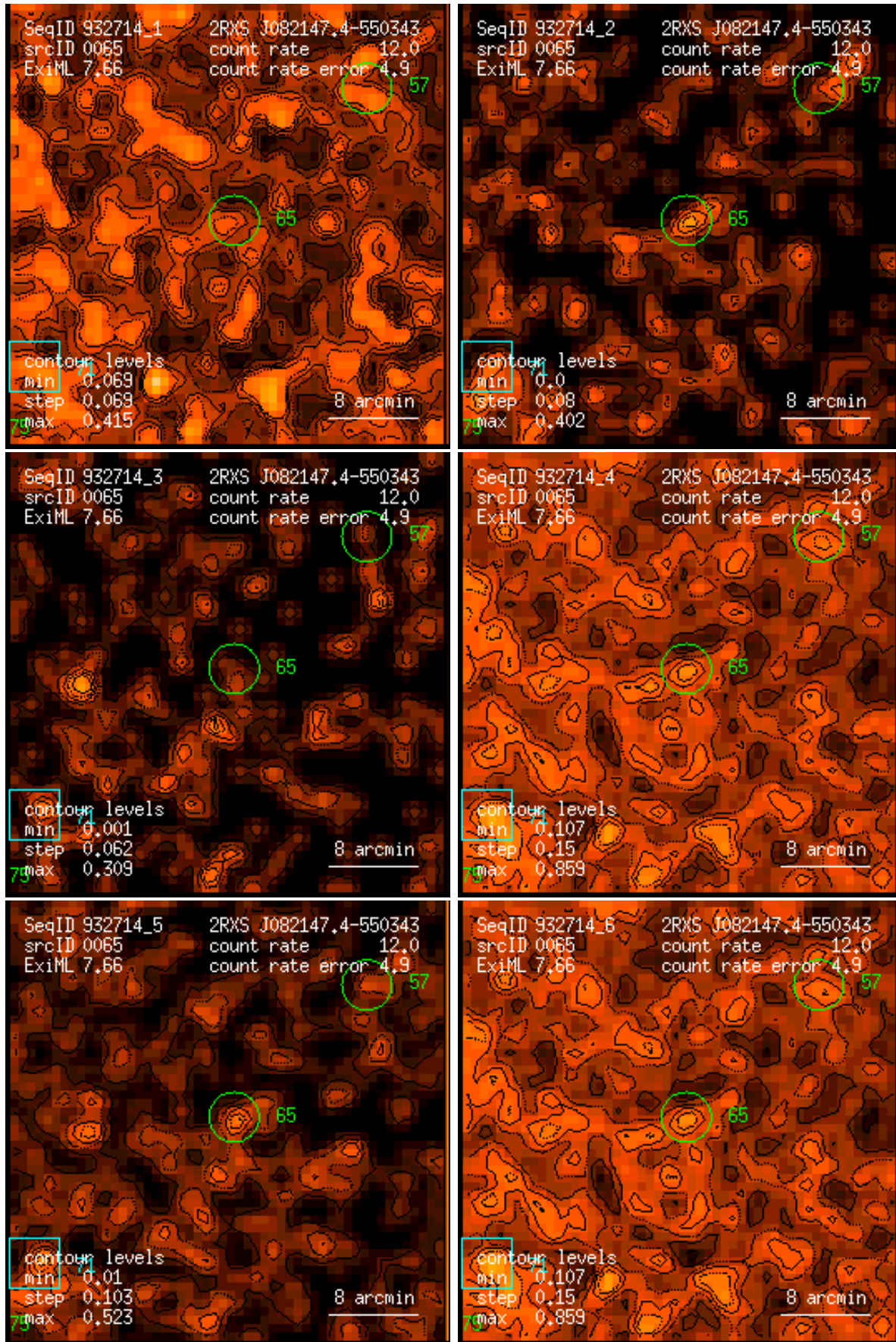
Figure 65: RASS 932714: detection 0065: band rate images, Gaussian filter: (1) PSPC channels 11 – 41, (2) 52 – 90, (3) 91 – 201, (4) 11 – 235, (5) 52 – 201, (6) 11 – 201. Broad band rates in counts/ks. Band rate contour levels in counts/ks/arcmin 2 .
