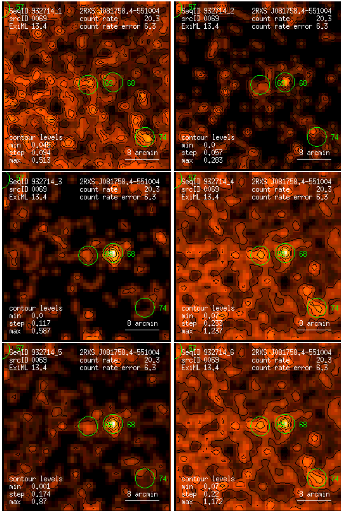
Figure 69: RASS 932714: detection 0069: band rate images, Gaussian filter: (1) PSPC channels 11 – 41, (2) 52 – 90, (3) 91 – 201, (4) 11 – 235, (5) 52 – 201, (6) 11 – 201. Broad band rates in counts/ks. Band rate contour levels in counts/ks/arcmin 2 .
