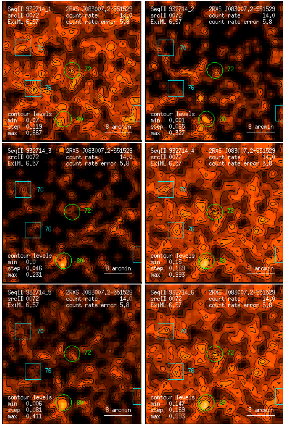
Figure 72: RASS 932714: detection 0072: band rate images, Gaussian filter: (1) PSPC channels 11 – 41, (2) 52 – 90, (3) 91 – 201, (4) 11 – 235, (5) 52 – 201, (6) 11 – 201. Broad band rates in counts/ks. Band rate contour levels in counts/ks/arcmin 2 .
