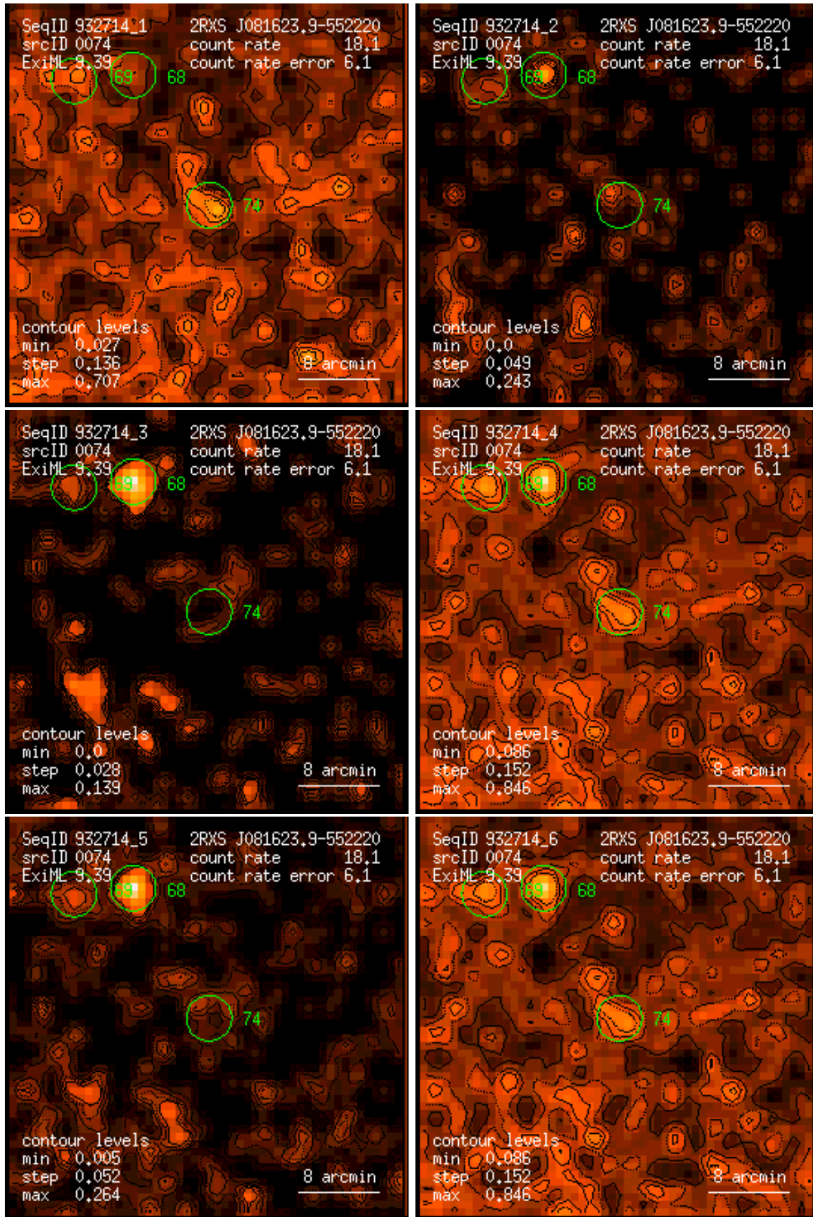
Figure 74: RASS 932714: detection 0074: band rate images, Gaussian filter: (1) PSPC channels 11 – 41, (2) 52 – 90, (3) 91 – 201, (4) 11 – 235, (5) 52 – 201, (6) 11 – 201. Broad band rates in counts/ks. Band rate contour levels in counts/ks/arcmin 2 .
