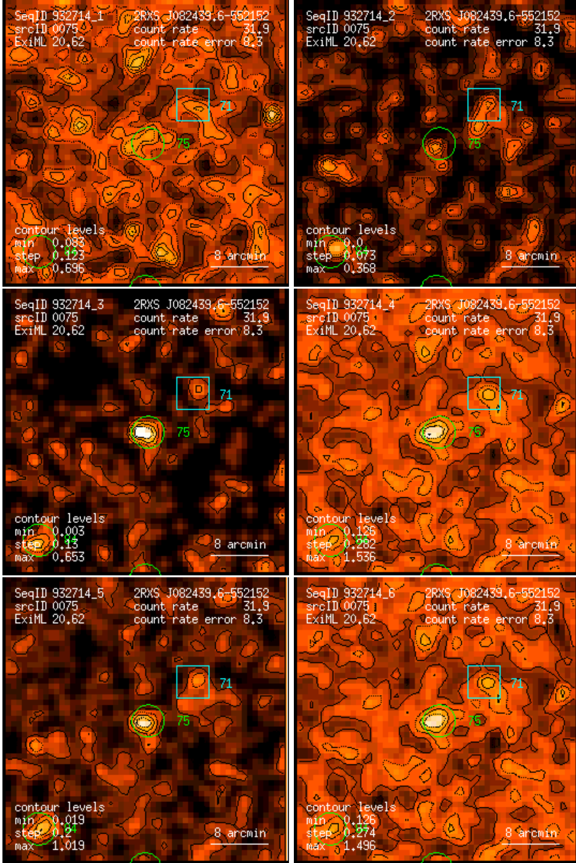
Figure 75: RASS 932714: detection 0075: band rate images, Gaussian filter: (1) PSPC channels 11 – 41, (2) 52 – 90, (3) 91 – 201, (4) 11 – 235, (5) 52 – 201, (6) 11 – 201. Broad band rates in counts/ks. Band rate contour levels in counts/ks/arcmin 2 .
