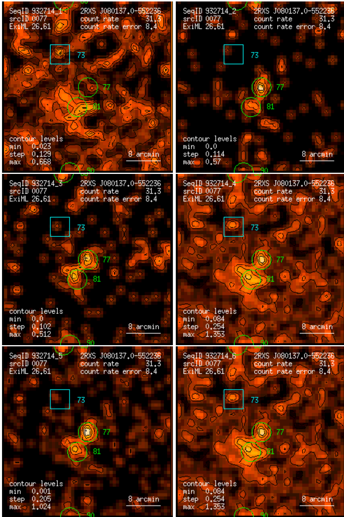
Figure 77: RASS 932714: detection 0077: band rate images, Gaussian filter: (1) PSPC channels 11 – 41, (2) 52 – 90, (3) 91 – 201, (4) 11 – 235, (5) 52 – 201, (6) 11 – 201. Broad band rates in counts/ks. Band rate contour levels in counts/ks/arcmin 2 .
