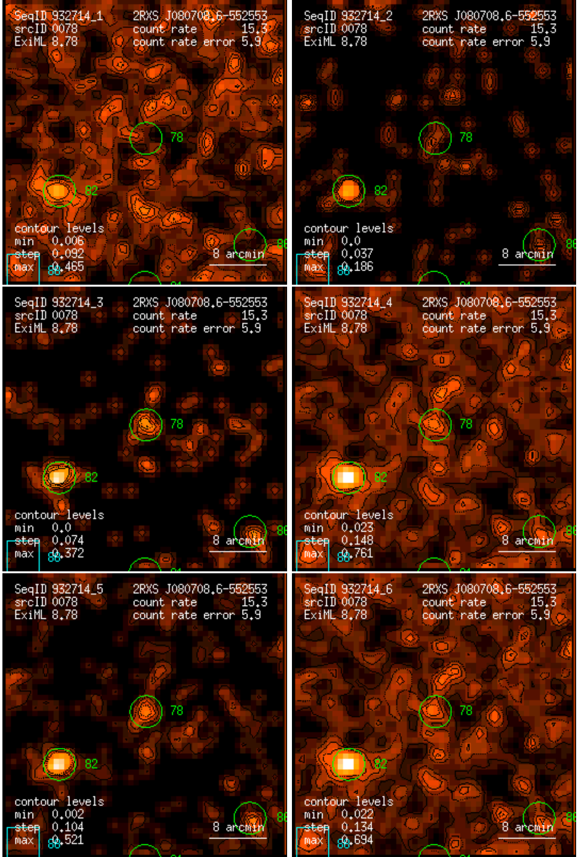
Figure 78: RASS 932714: detection 0078: band rate images, Gaussian filter: (1) PSPC channels 11 – 41, (2) 52 – 90, (3) 91 – 201, (4) 11 – 235, (5) 52 – 201, (6) 11 – 201. Broad band rates in counts/ks. Band rate contour levels in counts/ks/arcmin 2 .
