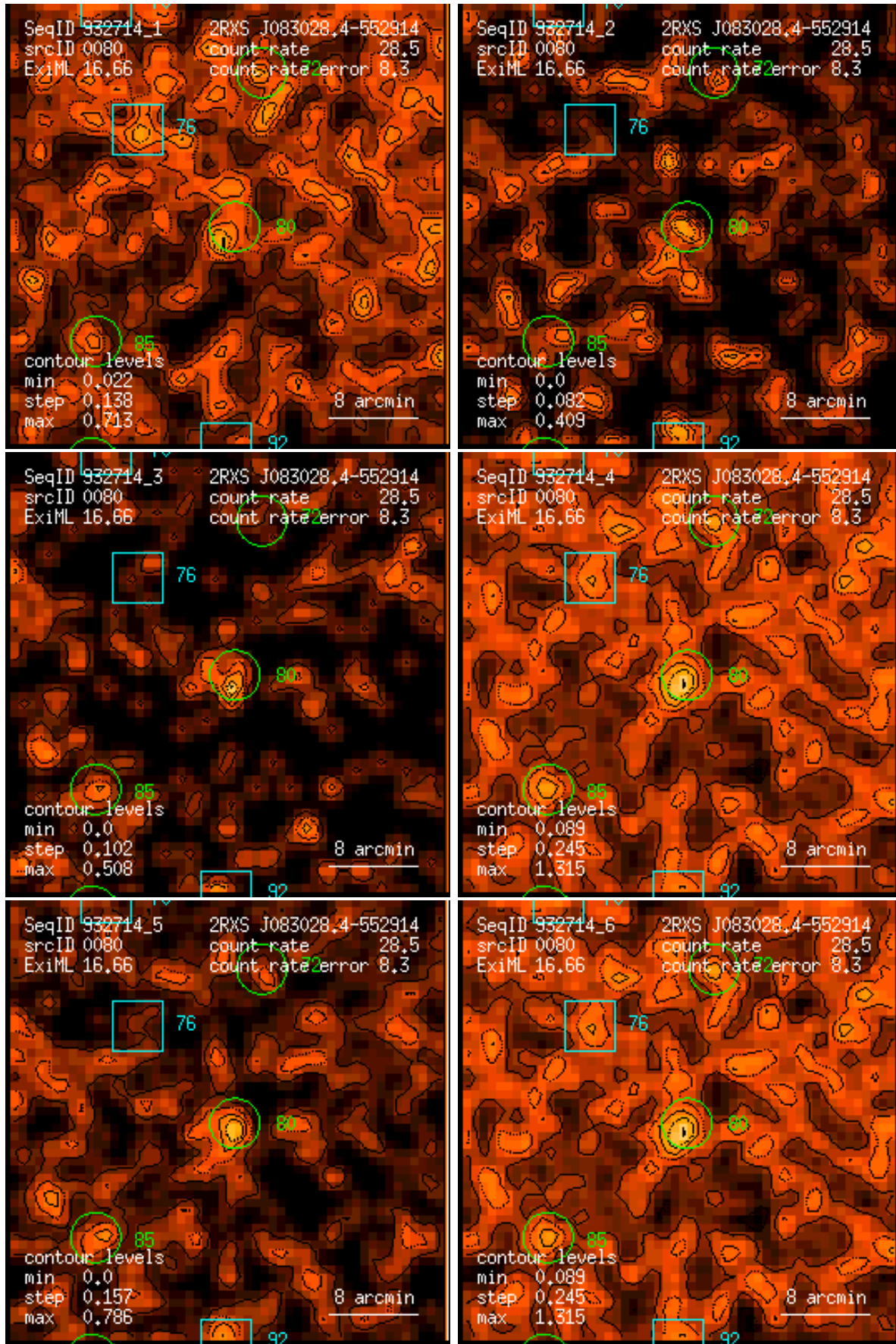
Figure 80: RASS 932714: detection 0080: band rate images, Gaussian filter: (1) PSPC channels 11 – 41, (2) 52 – 90, (3) 91 – 201, (4) 11 – 235, (5) 52 – 201, (6) 11 – 201. Broad band rates in counts/ks. Band rate contour levels in counts/ks/arcmin 2 .
