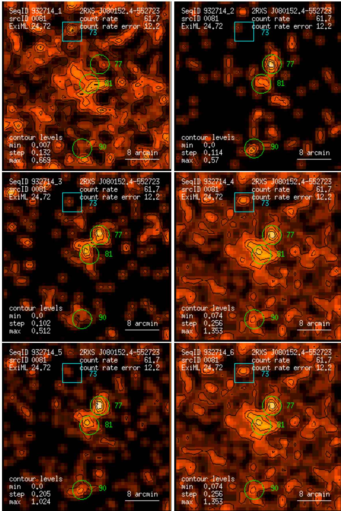
Figure 81: RASS 932714: detection 0081: band rate images, Gaussian filter: (1) PSPC channels 11 – 41, (2) 52 – 90, (3) 91 – 201, (4) 11 – 235, (5) 52 – 201, (6) 11 – 201. Broad band rates in counts/ks. Band rate contour levels in counts/ks/arcmin 2 .
