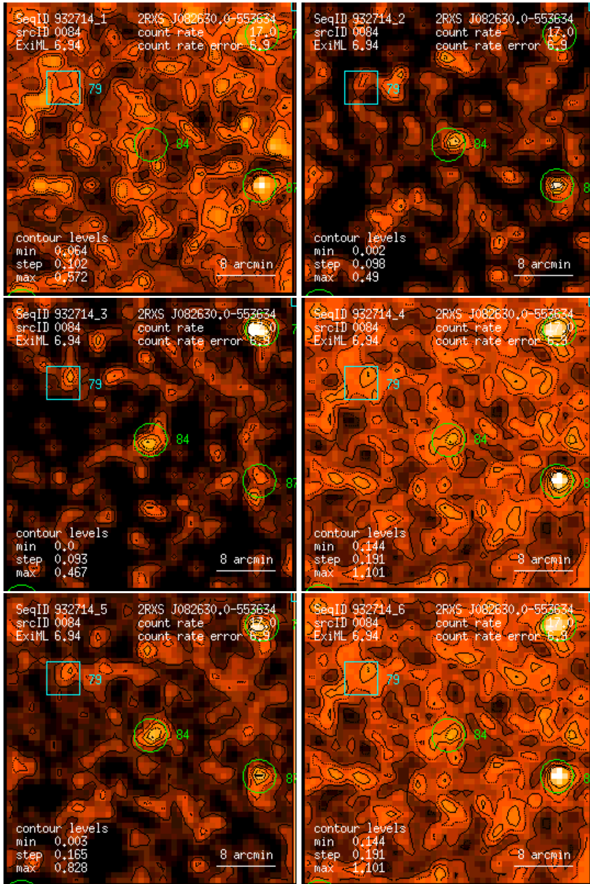
Figure 84: RASS 932714: detection 0084: band rate images, Gaussian filter: (1) PSPC channels 11 – 41, (2) 52 – 90, (3) 91 – 201, (4) 11 – 235, (5) 52 – 201, (6) 11 – 201. Broad band rates in counts/ks. Band rate contour levels in counts/ks/arcmin 2 .
