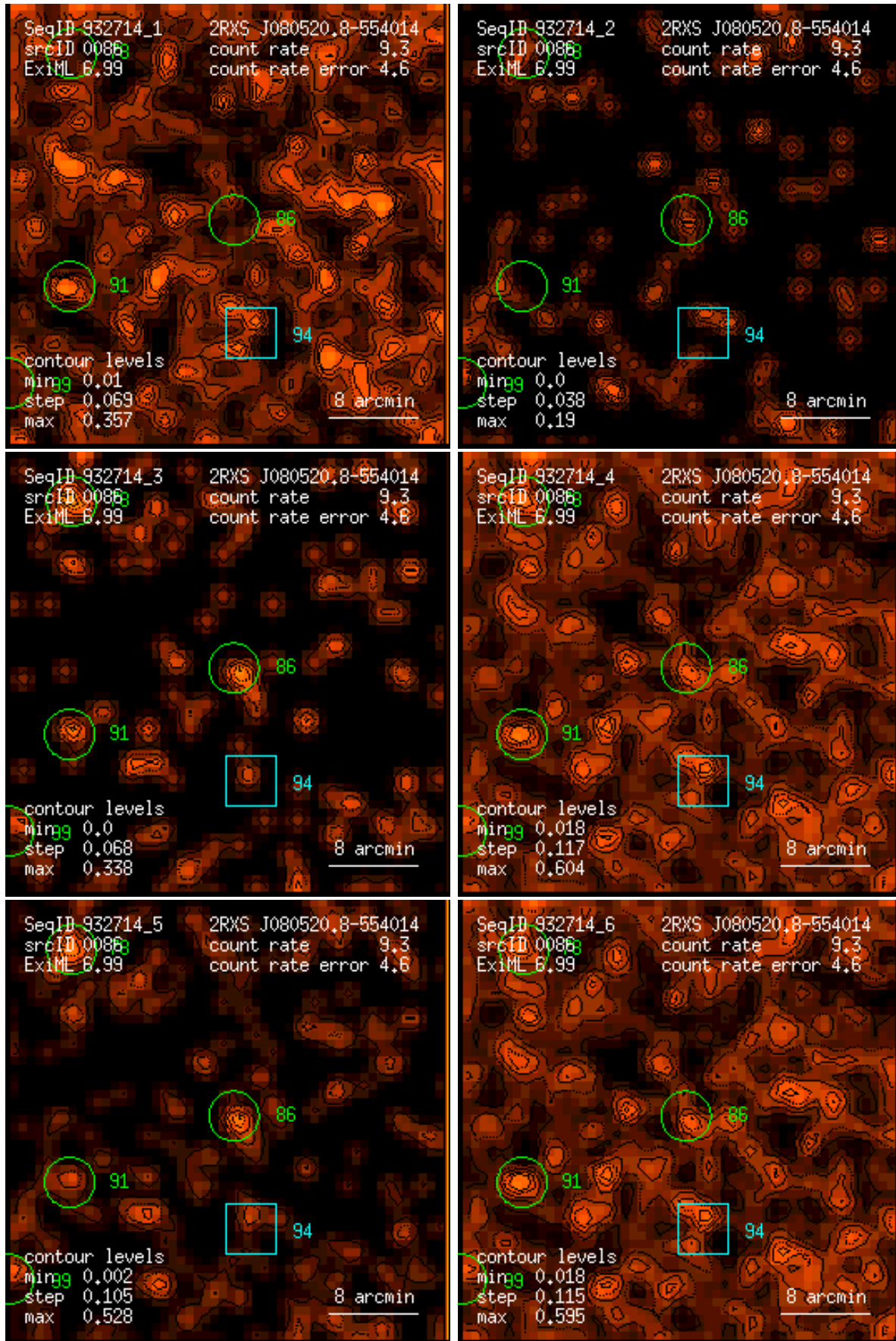
Figure 86: RASS 932714: detection 0086: band rate images, Gaussian filter: (1) PSPC channels 11 – 41, (2) 52 – 90, (3) 91 – 201, (4) 11 – 235, (5) 52 – 201, (6) 11 – 201. Broad band rates in counts/ks. Band rate contour levels in counts/ks/arcmin 2 .
