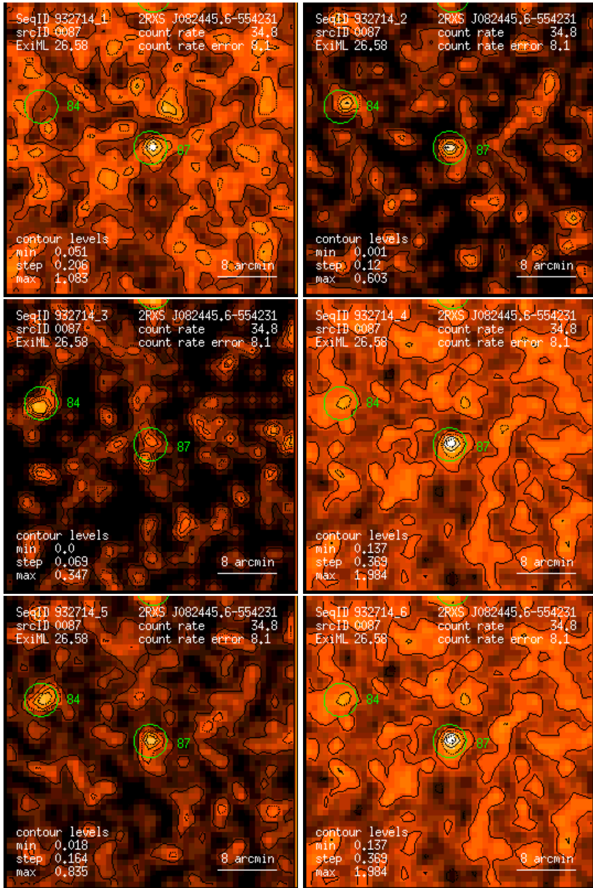
Figure 87: RASS 932714: detection 0087: band rate images, Gaussian filter: (1) PSPC channels 11 – 41, (2) 52 – 90, (3) 91 – 201, (4) 11 – 235, (5) 52 – 201, (6) 11 – 201. Broad band rates in counts/ks. Band rate contour levels in counts/ks/arcmin 2 .
