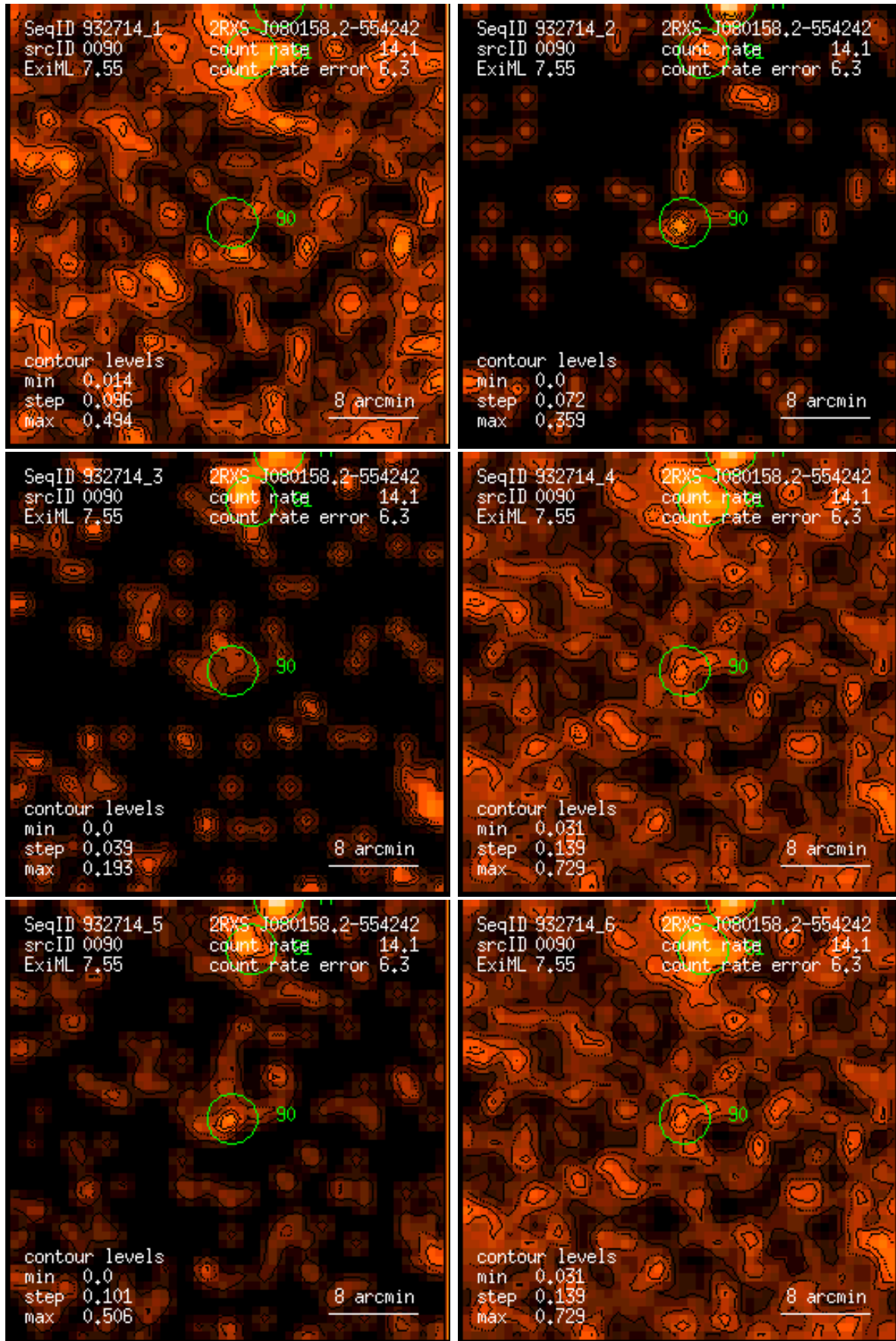
Figure 90: RASS 932714: detection 0090: band rate images, Gaussian filter: (1) PSPC channels 11 – 41, (2) 52 – 90, (3) 91 – 201, (4) 11 – 235, (5) 52 – 201, (6) 11 – 201. Broad band rates in counts/ks. Band rate contour levels in counts/ks/arcmin 2 .
