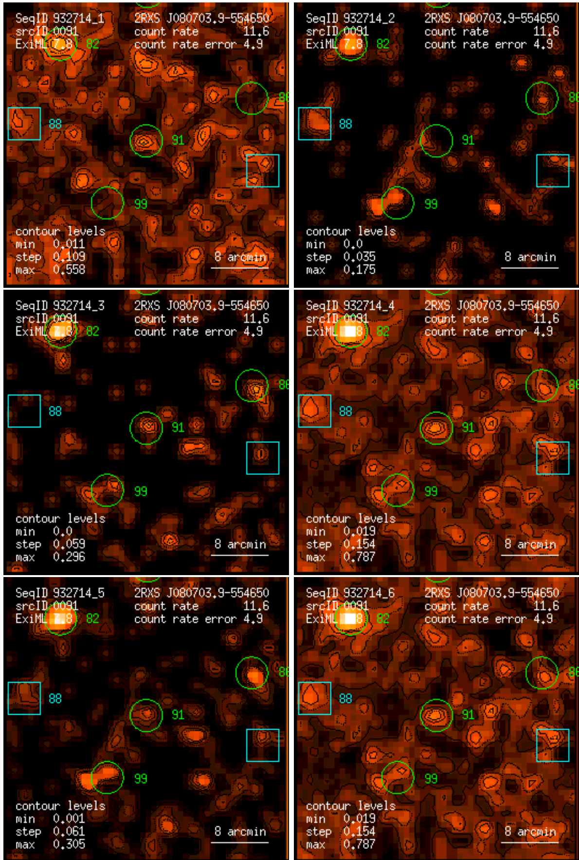
Figure 91: RASS 932714: detection 0091: band rate images, Gaussian filter: (1) PSPC channels 11 – 41, (2) 52 – 90, (3) 91 – 201, (4) 11 – 235, (5) 52 – 201, (6) 11 – 201. Broad band rates in counts/ks. Band rate contour levels in counts/ks/arcmin 2 .
