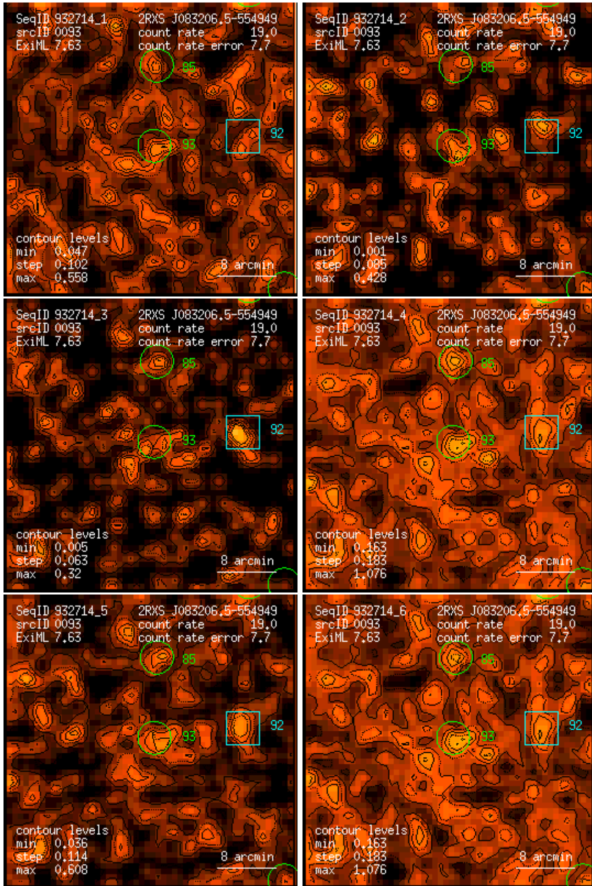
Figure 93: RASS 932714: detection 0093: band rate images, Gaussian filter: (1) PSPC channels 11 – 41, (2) 52 – 90, (3) 91 – 201, (4) 11 – 235, (5) 52 – 201, (6) 11 – 201. Broad band rates in counts/ks. Band rate contour levels in counts/ks/arcmin 2 .
