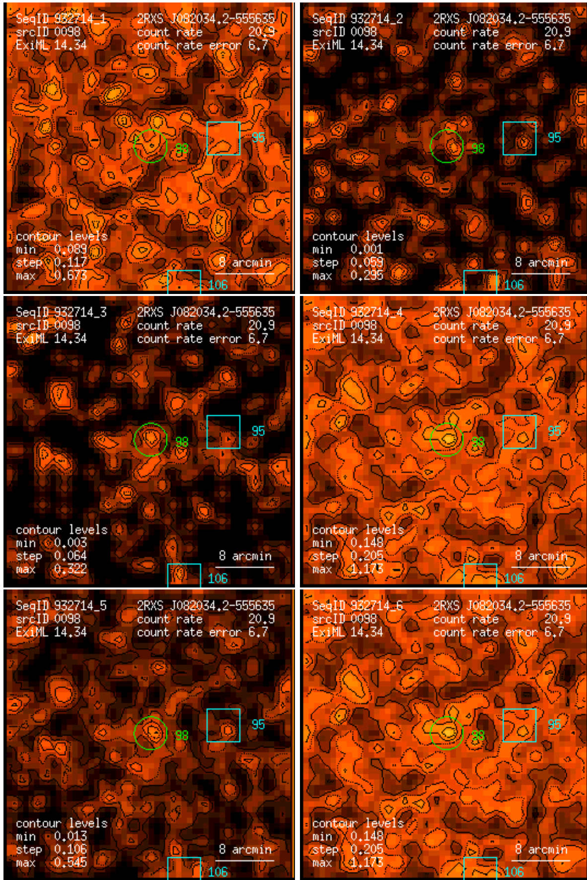
Figure 98: RASS 932714: detection 0098: band rate images, Gaussian filter: (1) PSPC channels 11 – 41, (2) 52 – 90, (3) 91 – 201, (4) 11 – 235, (5) 52 – 201, (6) 11 – 201. Broad band rates in counts/ks. Band rate contour levels in counts/ks/arcmin 2 .
