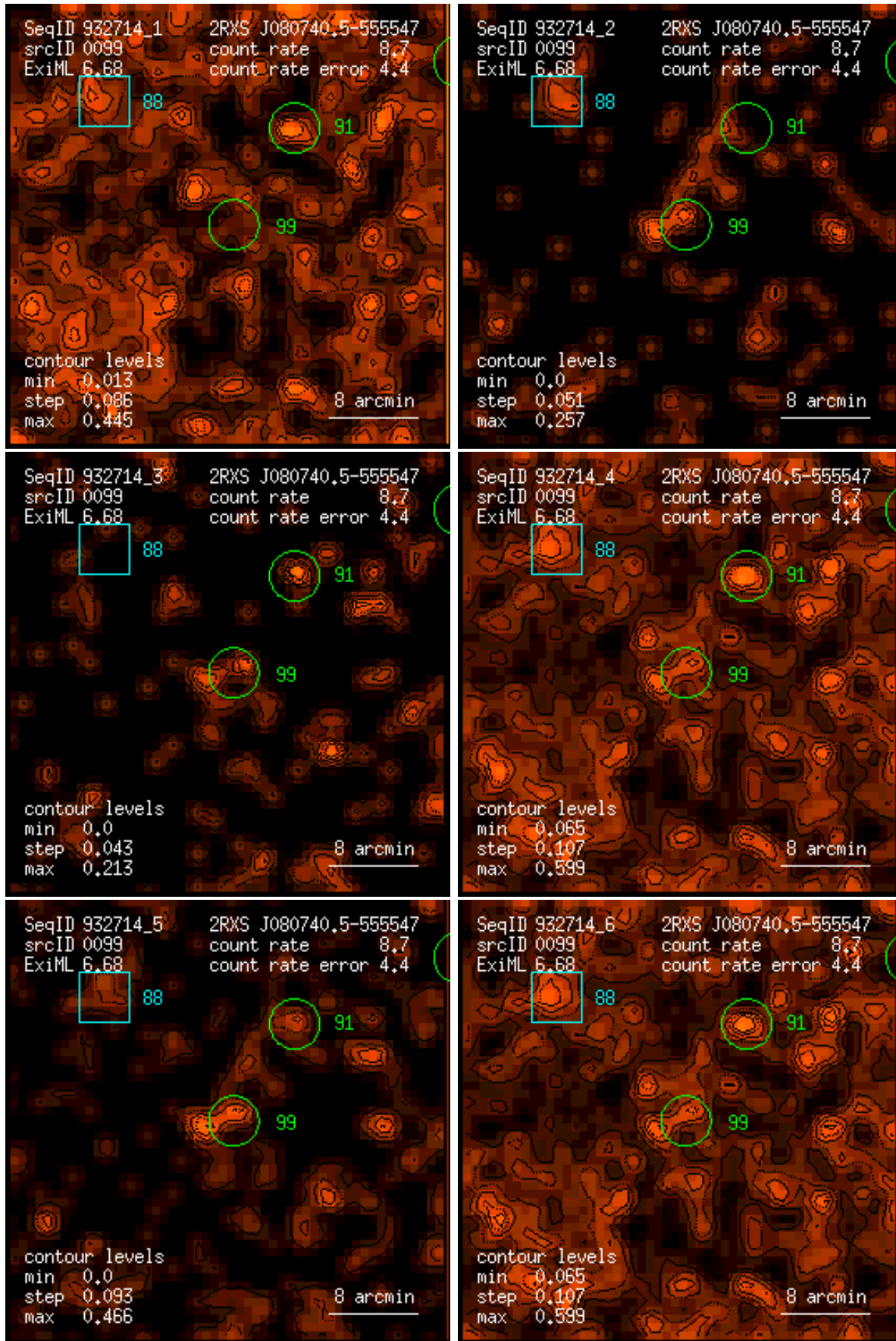
Figure 99: RASS 932714: detection 0099: band rate images, Gaussian filter: (1) PSPC channels 11 – 41, (2) 52 – 90, (3) 91 – 201, (4) 11 – 235, (5) 52 – 201, (6) 11 – 201. Broad band rates in counts/ks. Band rate contour levels in counts/ks/arcmin 2 .
