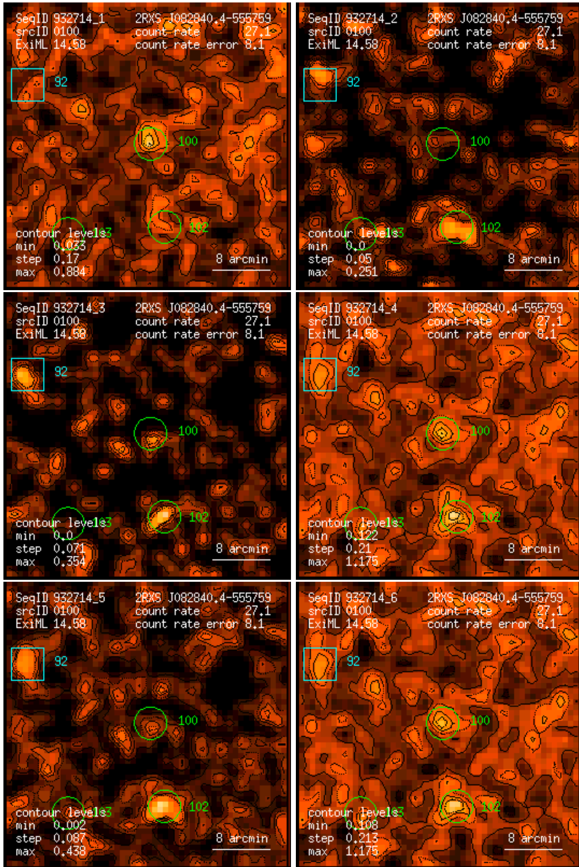
Figure 100: RASS 932714: detection 0100: band rate images, Gaussian filter: (1) PSPC channels 11 – 41, (2) 52 – 90, (3) 91 – 201, (4) 11 – 235, (5) 52 – 201, (6) 11 – 201. Broad band rates in counts/ks. Band rate contour levels in counts/ks/arcmin 2 .
