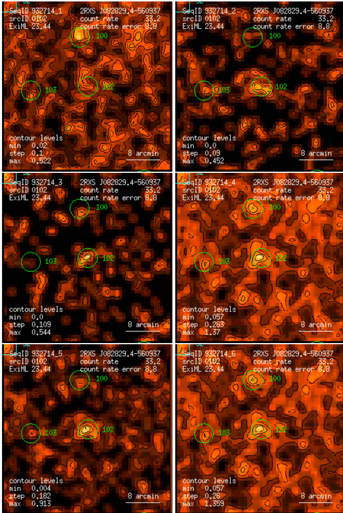
Figure 102: RASS 932714: detection 0102: band rate images, Gaussian filter: (1) PSPC channels 11 – 41, (2) 52 – 90, (3) 91 – 201, (4) 11 – 235, (5) 52 – 201, (6) 11 – 201. Broad band rates in counts/ks. Band rate contour levels in counts/ks/arcmin 2 .
