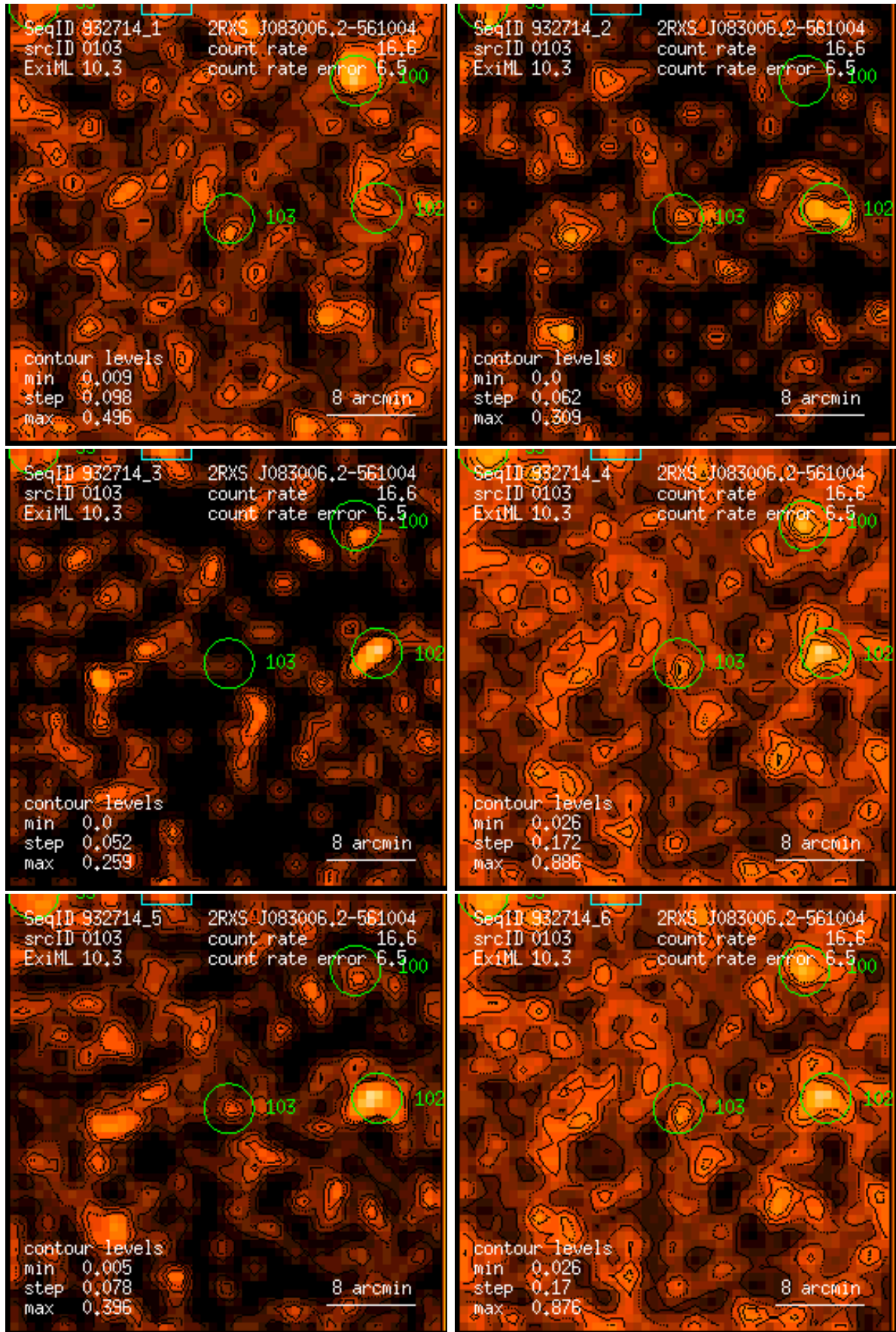
Figure 103: RASS 932714: detection 0103: band rate images, Gaussian filter: (1) PSPC channels 11 – 41, (2) 52 – 90, (3) 91 – 201, (4) 11 – 235, (5) 52 – 201, (6) 11 – 201. Broad band rates in counts/ks. Band rate contour levels in counts/ks/arcmin 2 .
