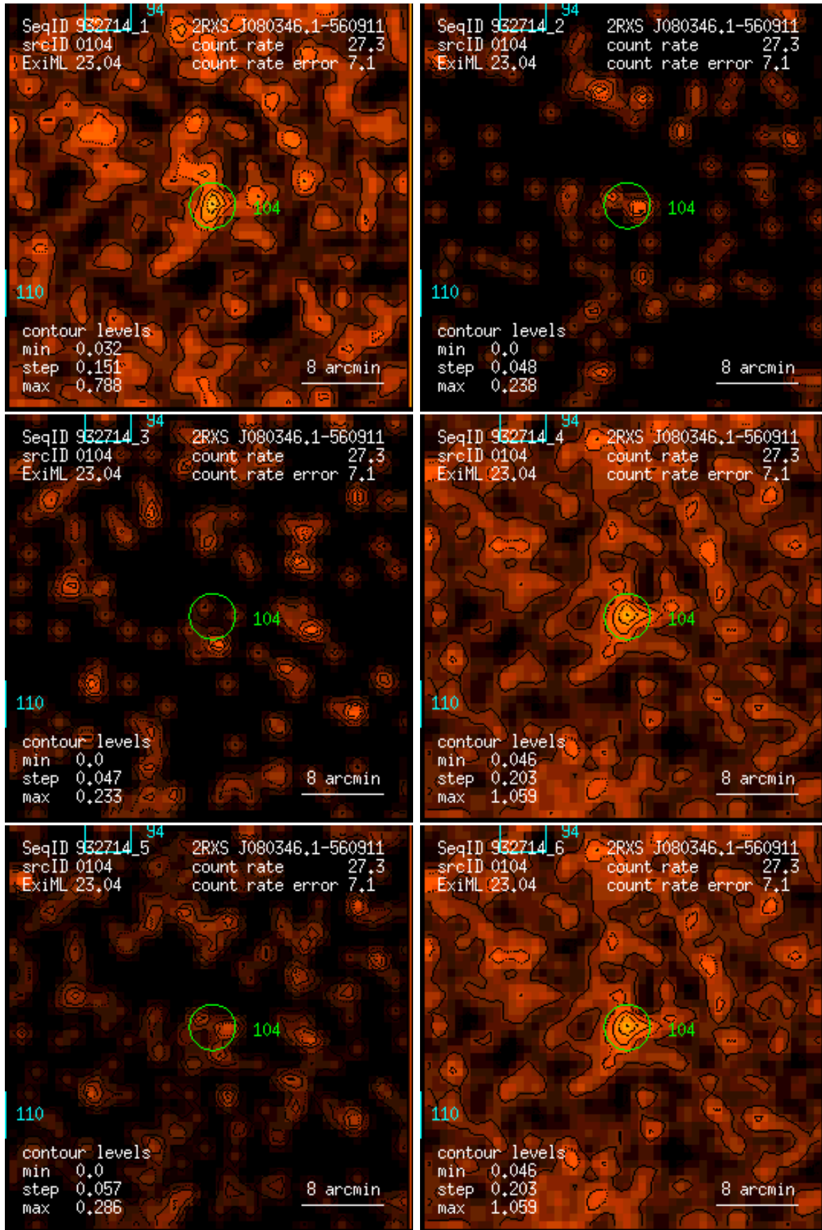
Figure 104: RASS 932714: detection 0104: band rate images, Gaussian filter: (1) PSPC channels 11 – 41, (2) 52 – 90, (3) 91 – 201, (4) 11 – 235, (5) 52 – 201, (6) 11 – 201. Broad band rates in counts/ks. Band rate contour levels in counts/ks/arcmin 2 .
